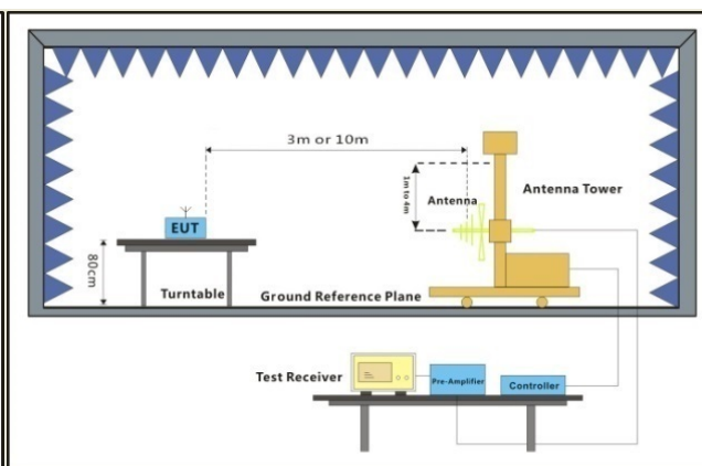
30MHz-1GHz
