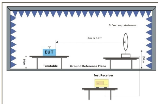
Below 30MHz
