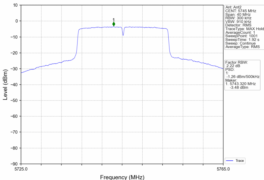
802.11n(HT20)_LCH_5745MHz_Ant2_NTNV
