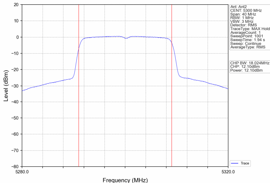
802.11ac(VHT20)_MCH_5300MHz_Ant2_NTNV
