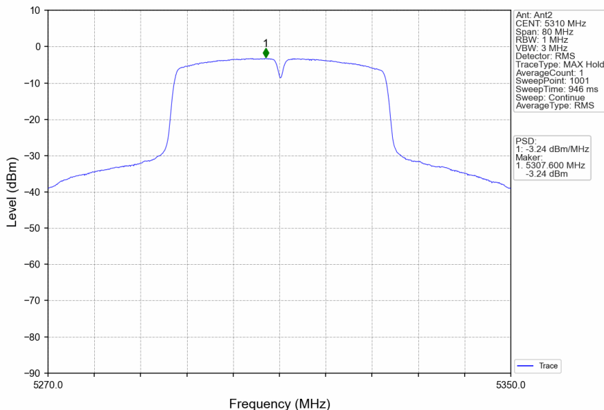
802.11n(HT40)_HCH_5310MHz_Ant2_NTNV
