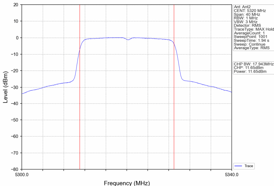
802.11ac(VHT20)_HCH_5320MHz_Ant2_NTNV
