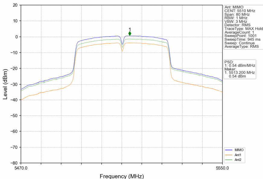
802.11n(HT40)_LCH_5510MHz_MIMO_NTNV
