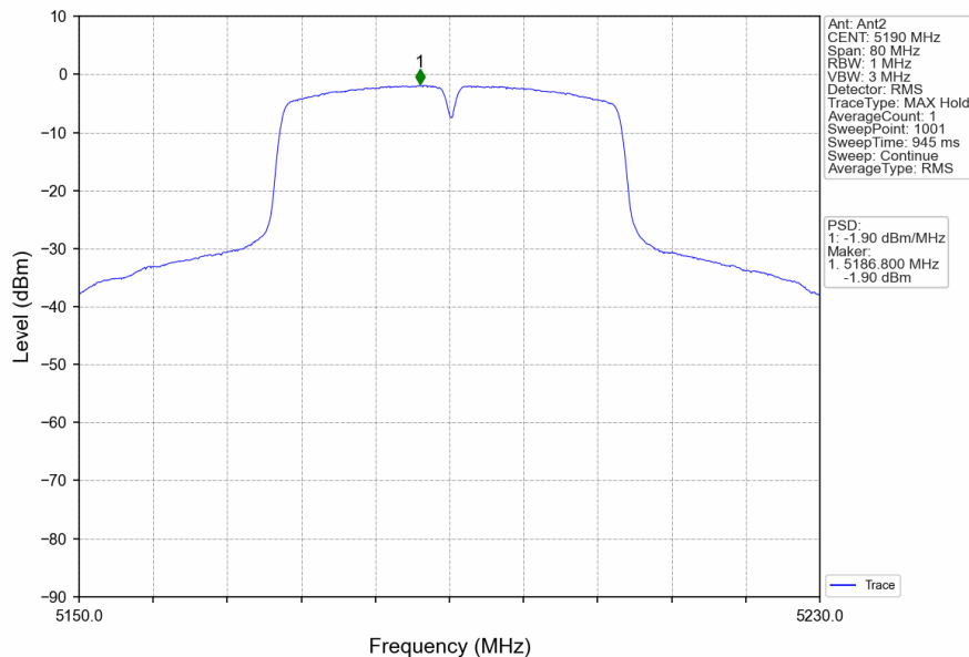
802.11n(HT40)_LCH_5190MHz_MIMO_NTNV
