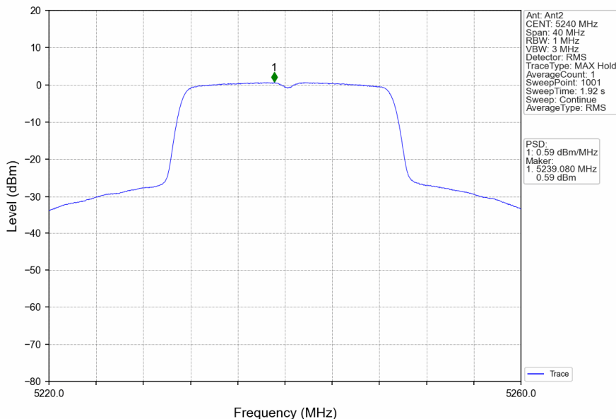
802.11n(HT20)_HCH_5240MHz_Ant2_NTNV
