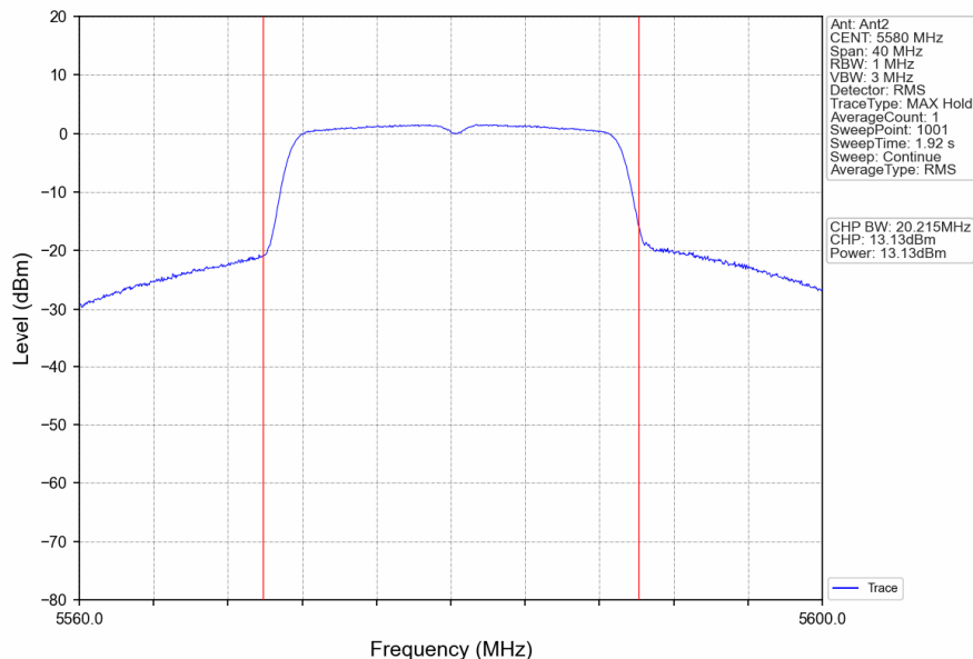
802.11n(HT20)_MCH_5580MHz_Ant2_NTNV
