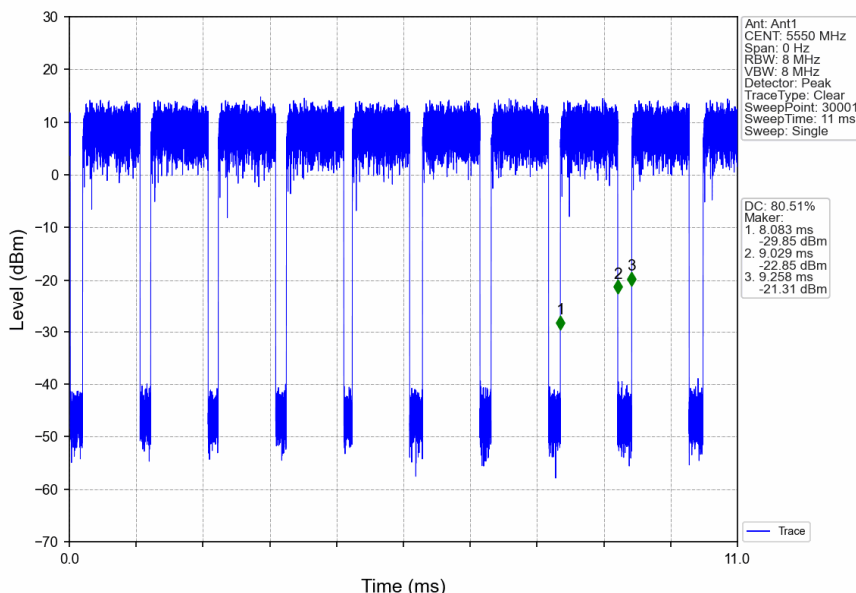
802.11n(HT40)_MCH_5550MHz_Ant1_NTNV
