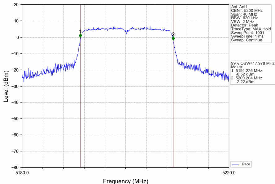
802.11n(HT20)_MCH_5200MHz_Ant1_NTNV
