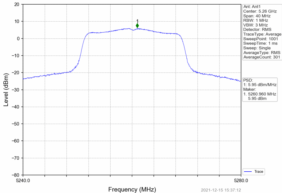
802.11ac(VHT20)_LCH_5260MHz_Ant1_NTNV
