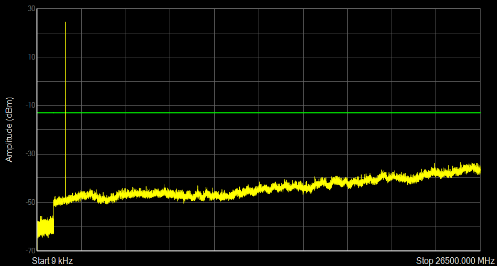
Band66 QAM16 BW=1.4MHz Channel=131979 RB Size=6 Position=#0
