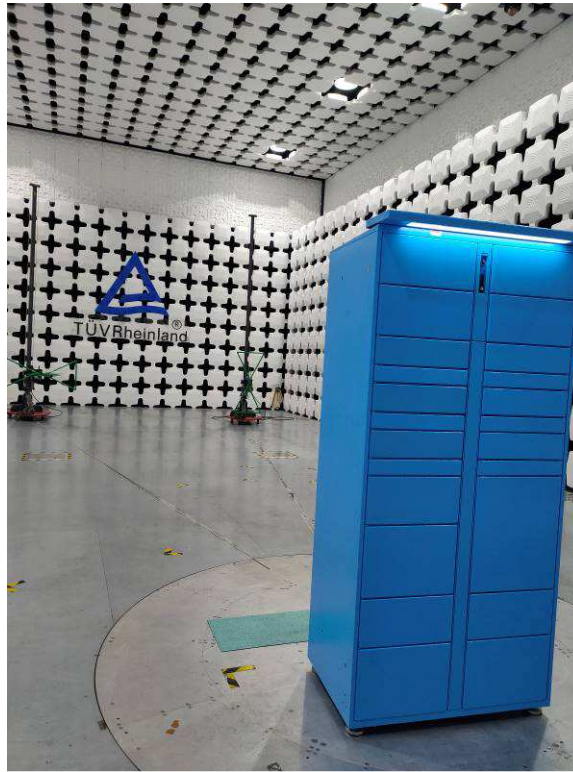
Photograph 1: Set-up photo for Radiated Emission, Below 1GHz
