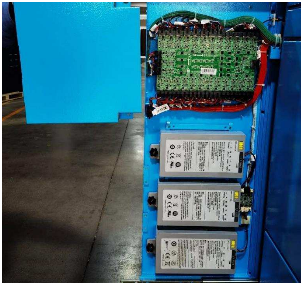
Internal view with 3pcs batteries
