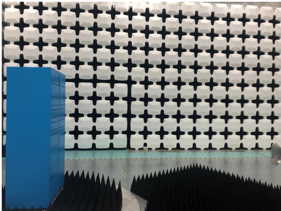
Photograph 2: Set-up for Radiated Emission, 1GHz to 6GHz
