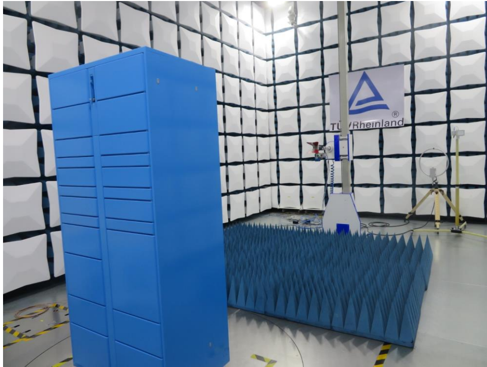
Photograph 3: Set-up for Radiated Emission, Above 6GHz
