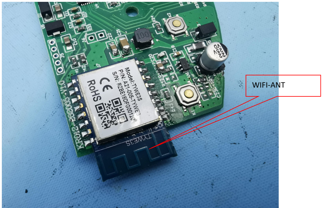
INTERNAL VIEW-4 OF EUT
