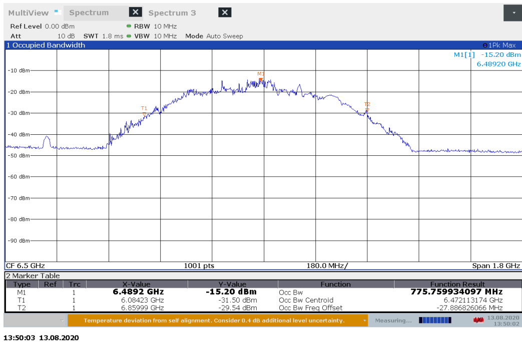
Figure 8.6-2: 99% occupied bandwidth
