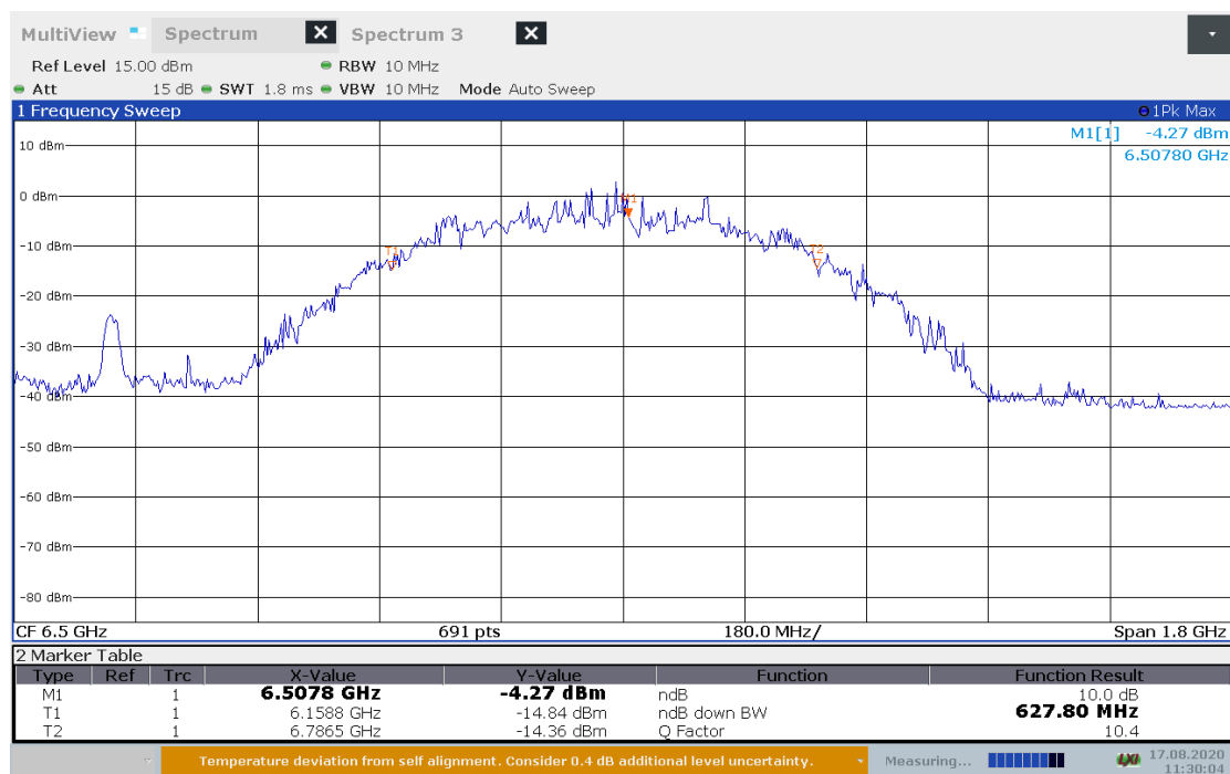
Figure 8.6-1: 10 dB occupied bandwidth
