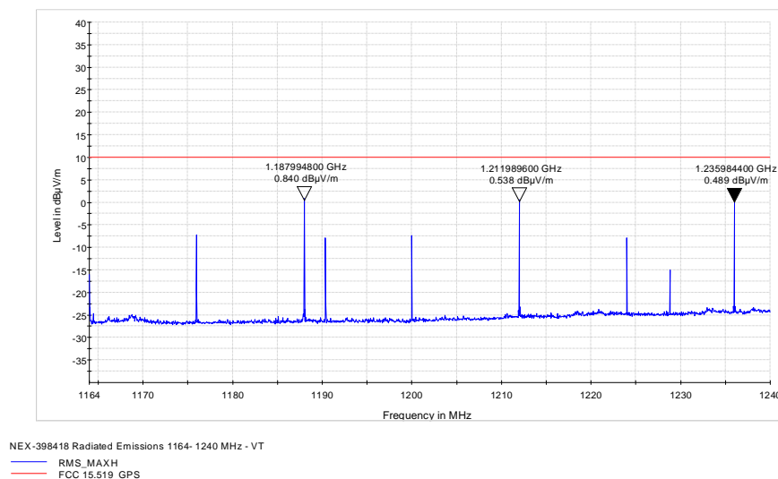
Figure 8.7-1: Spurious emissions within 1164-1240 MHz
