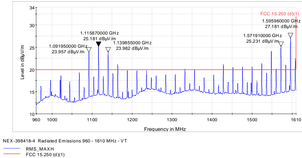
Figure 8.5-2: Spurious emissions 960 – 1610 MHz
