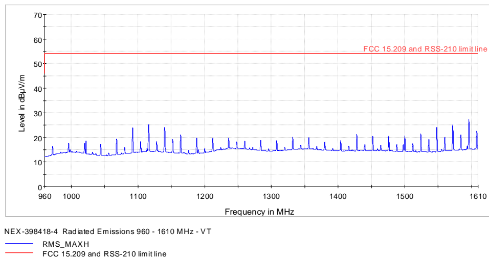
Figure 8.5-3: Digital circuitry Spurious emissions 960 MHz – 1.61 GHz
