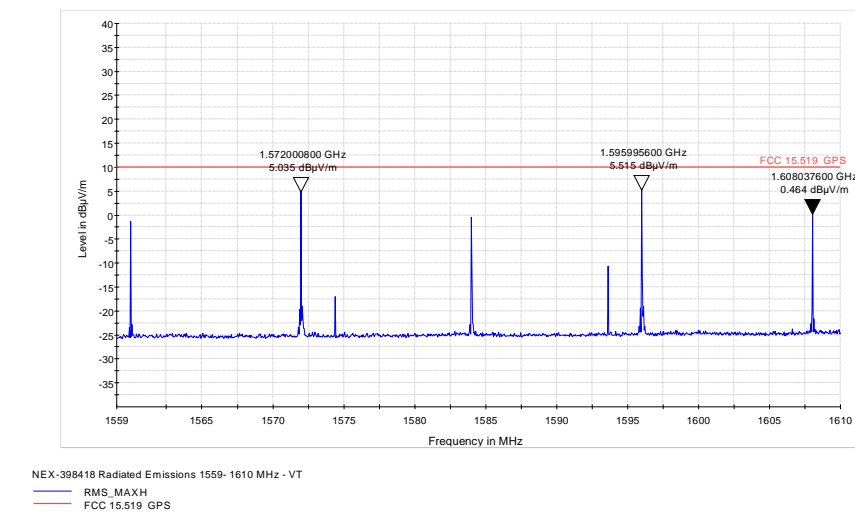
Figure 8.7-2: Spurious emissions within 1559-1610 MHz
