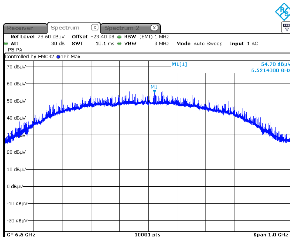
Plot 8.4-1: Peak emissions plot
