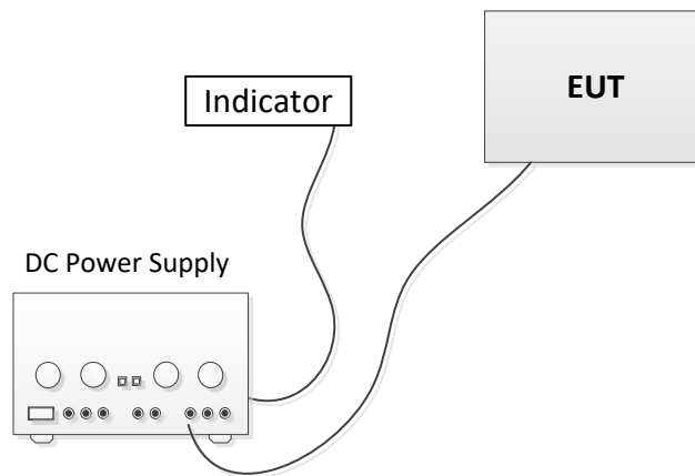
Figure 5.6-1: Radiated testing block diagram
