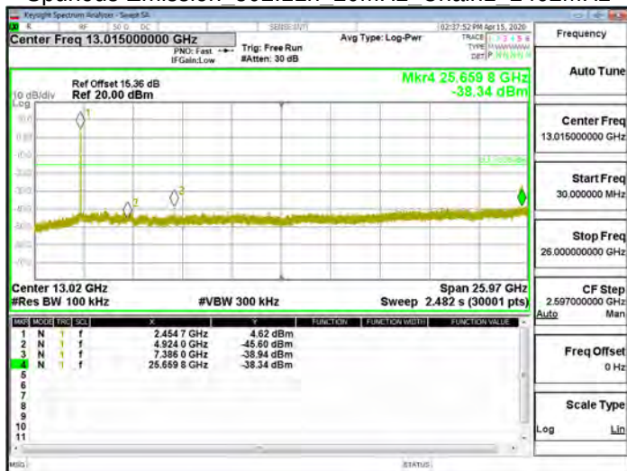
Spurious Emission 802.11n 20MHz Chain1 2462MHz
