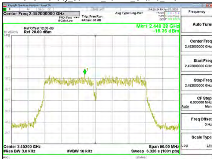
Power Density 802.11n 40MHz Chain0 2452MHz
