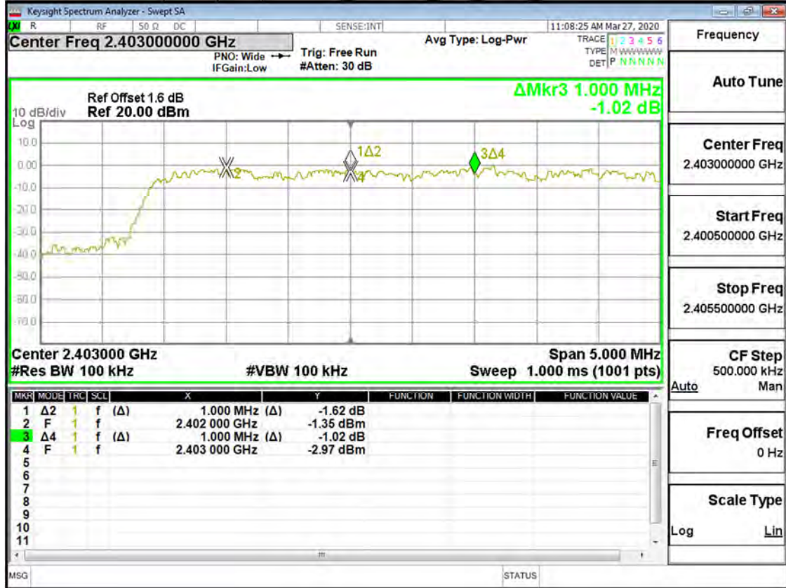
Frequency Separation 8DPSK 3M DH5 CH0CH1CH2
