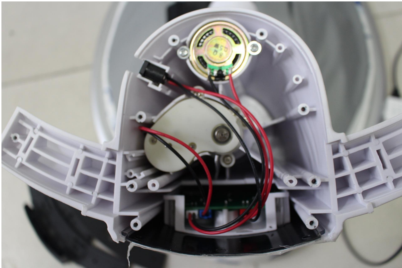
Internal photo
