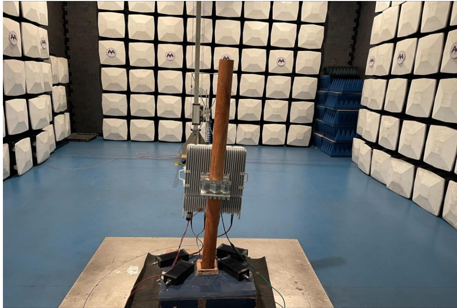
Test Setup photograph
