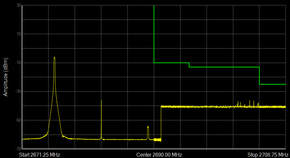
Band41 QAM16 BW=15MHz Channel=41515 RB Size=1 Position=#0
