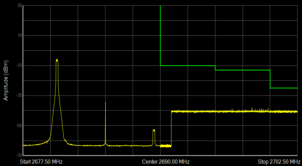
Band41 QAM16 BW=10MHz Channel=41540 RB Size=1 Position=#0
