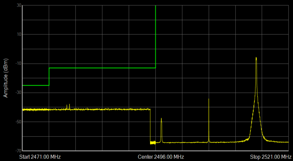
Band41 QPSK BW=20MHz Channel=39750 RB Size=1 Position=#Max
