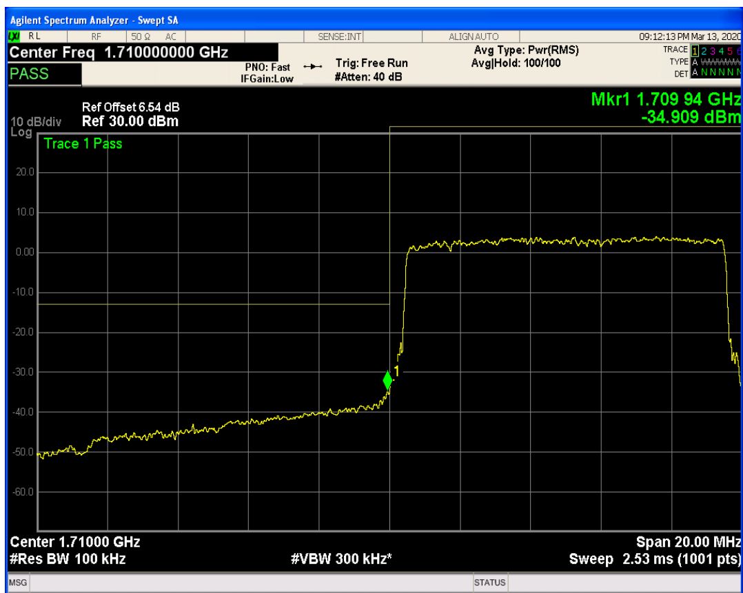
LTE Band4 QPSK BW=10MHz Channel=20000 RB Size=1 Position=#Max
