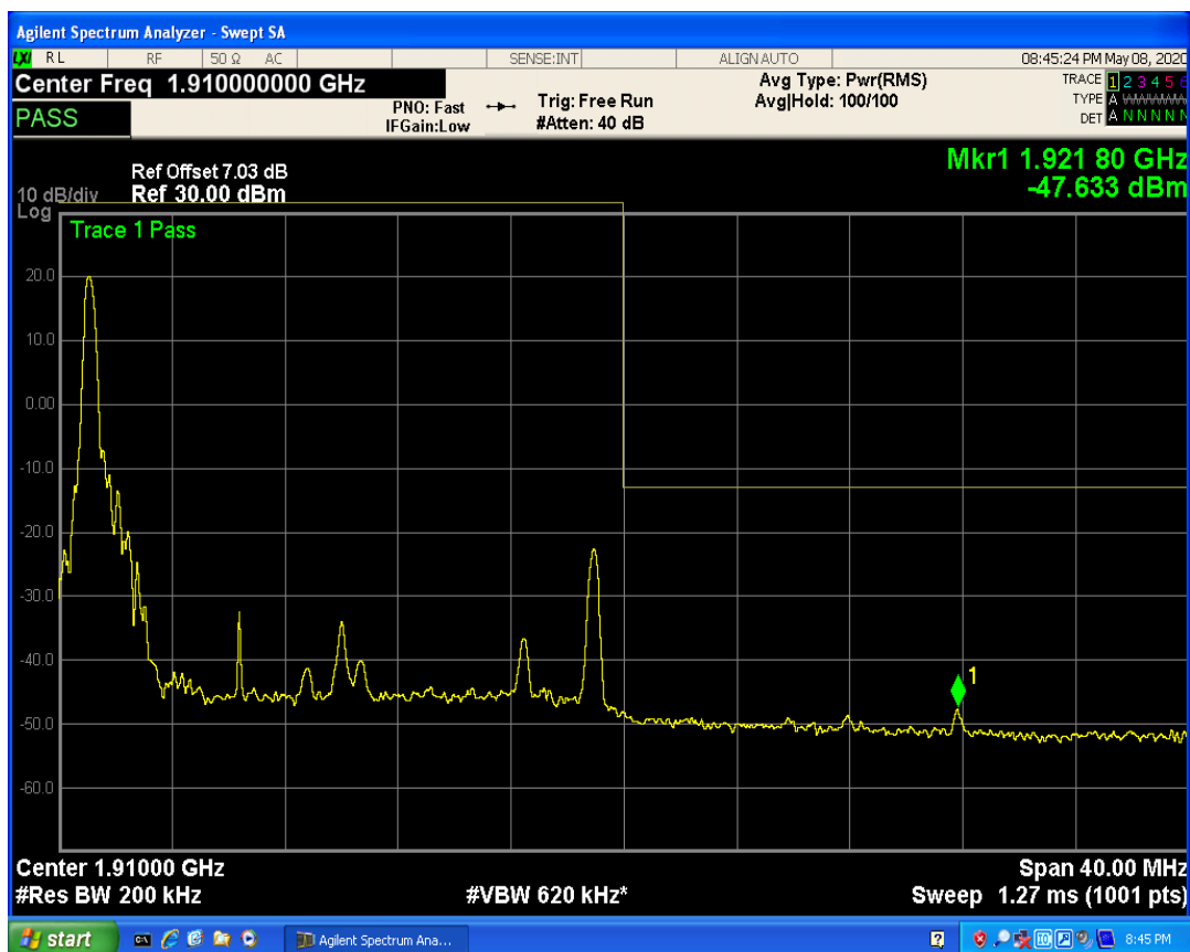
LTE Band2 QAM16 BW=20MHz Channel=19100 RB Size=1 Position=#Max
