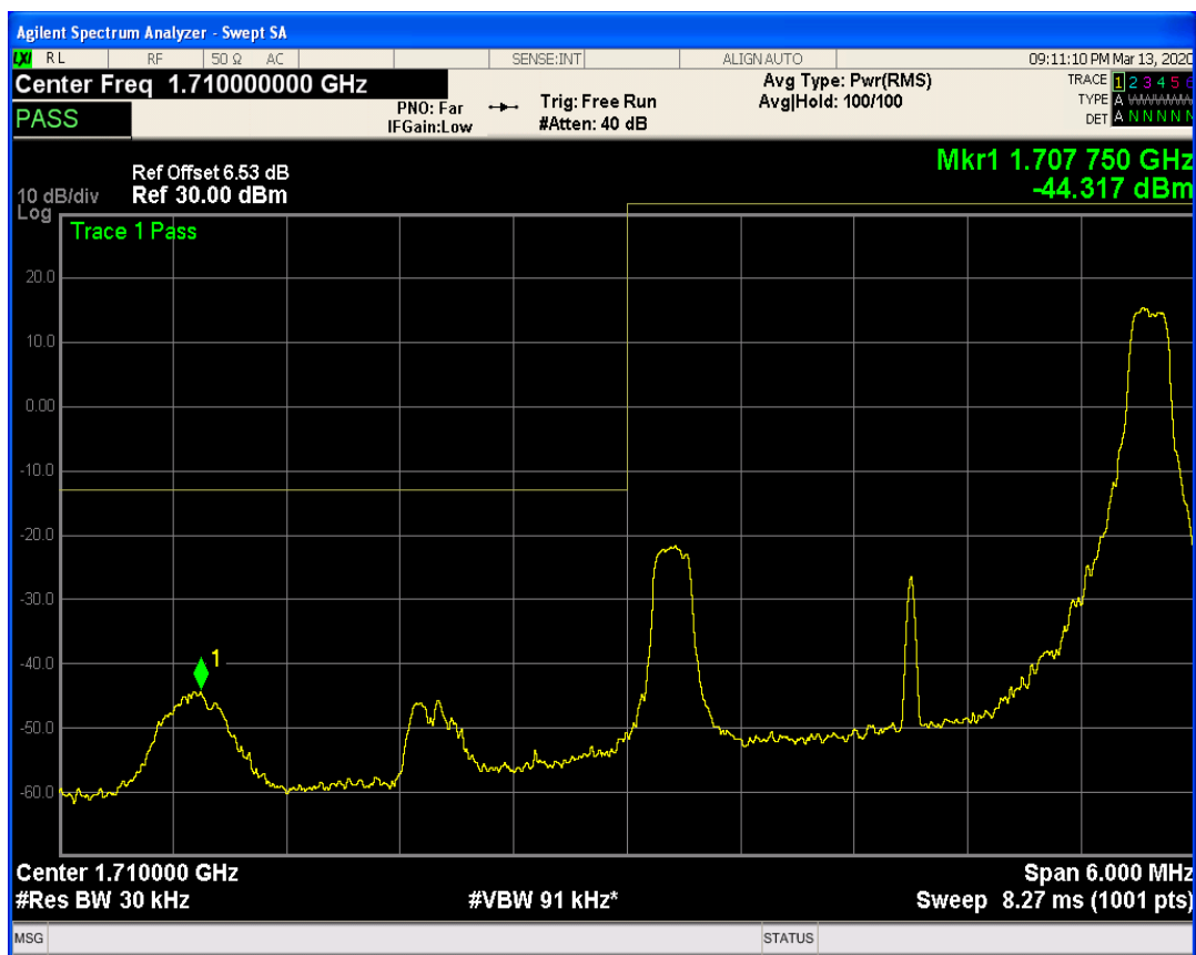
LTE Band4 QPSK BW=3MHz Channel=19965 RB Size=15 Position=#0
