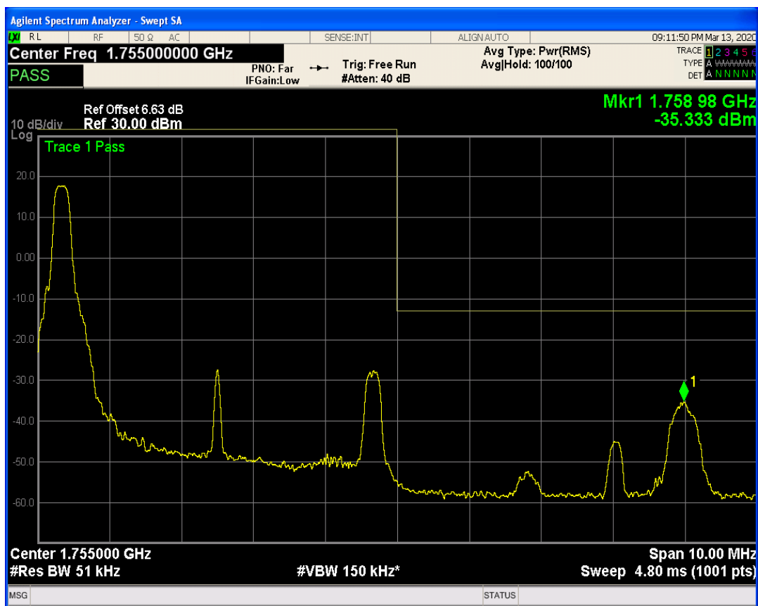
LTE Band4 QPSK BW=5MHz Channel=20375 RB Size=1 Position=#Max
