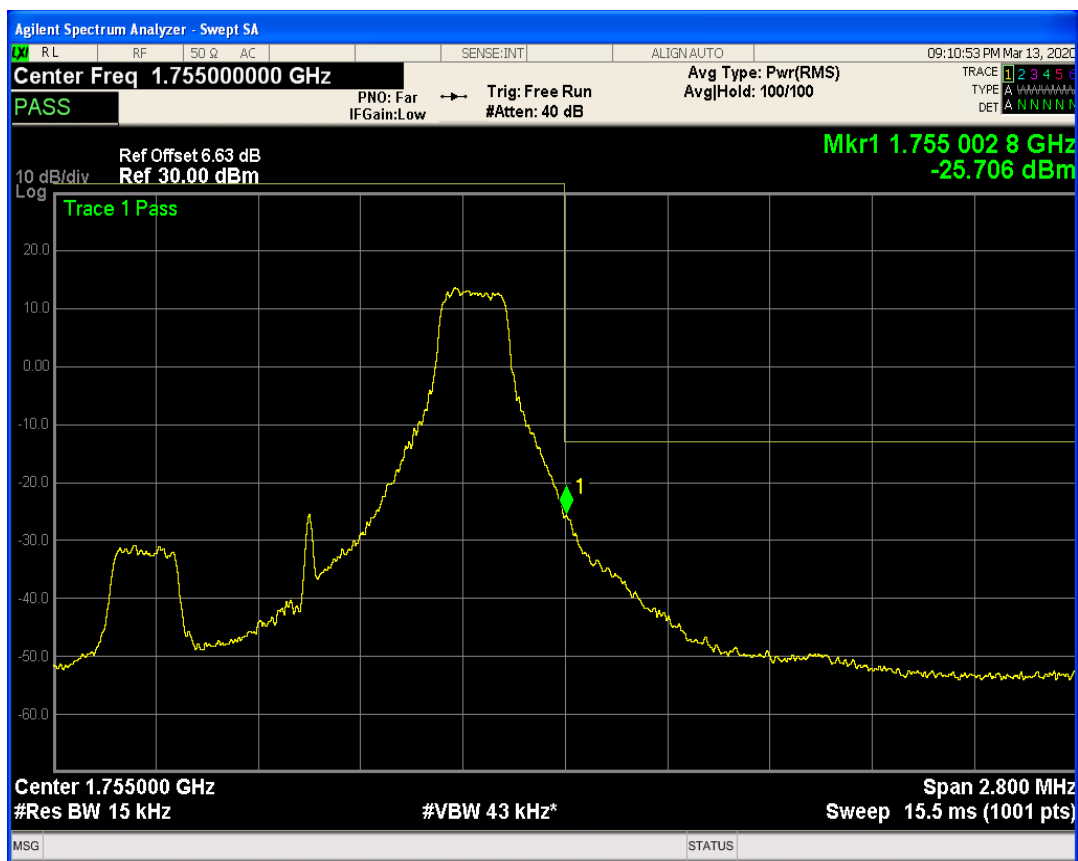
LTE Band4 QPSK BW=1.4MHz Channel=20393 RB Size=1 Position=#0
