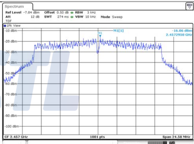
802.11g / 2 457 MHz
