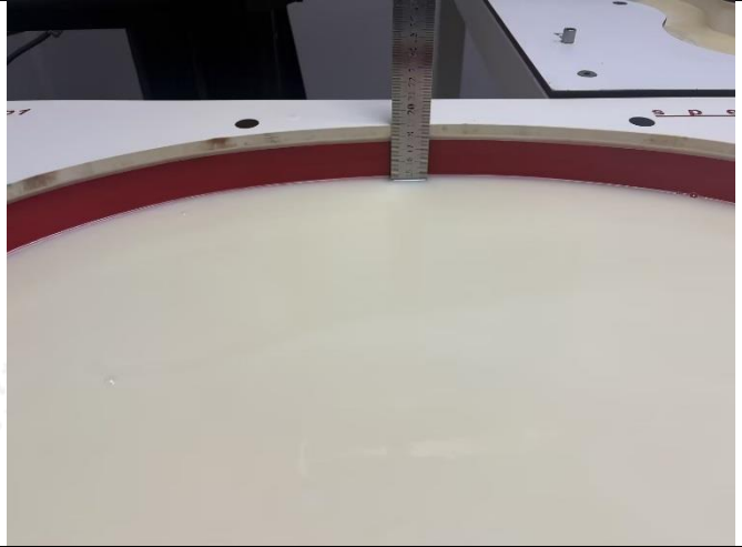
Photo 2: Tissue Simulant Liquid for Head 3000-8000 Mhz
