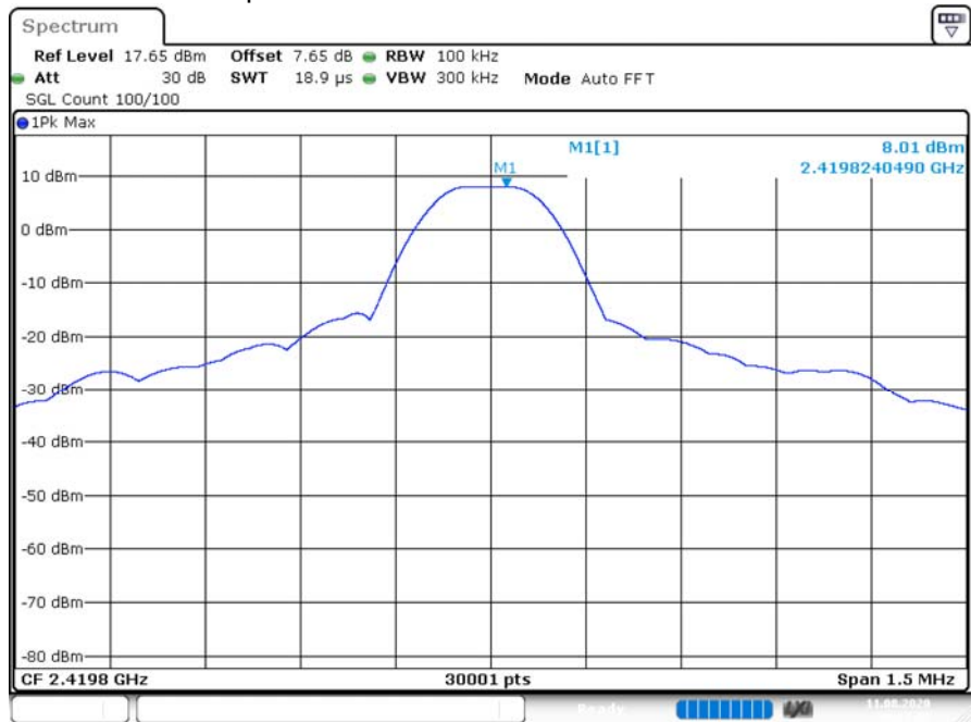
Tx. Spurious NVNT GFSK 2419.8MHz Ant1 Ref
