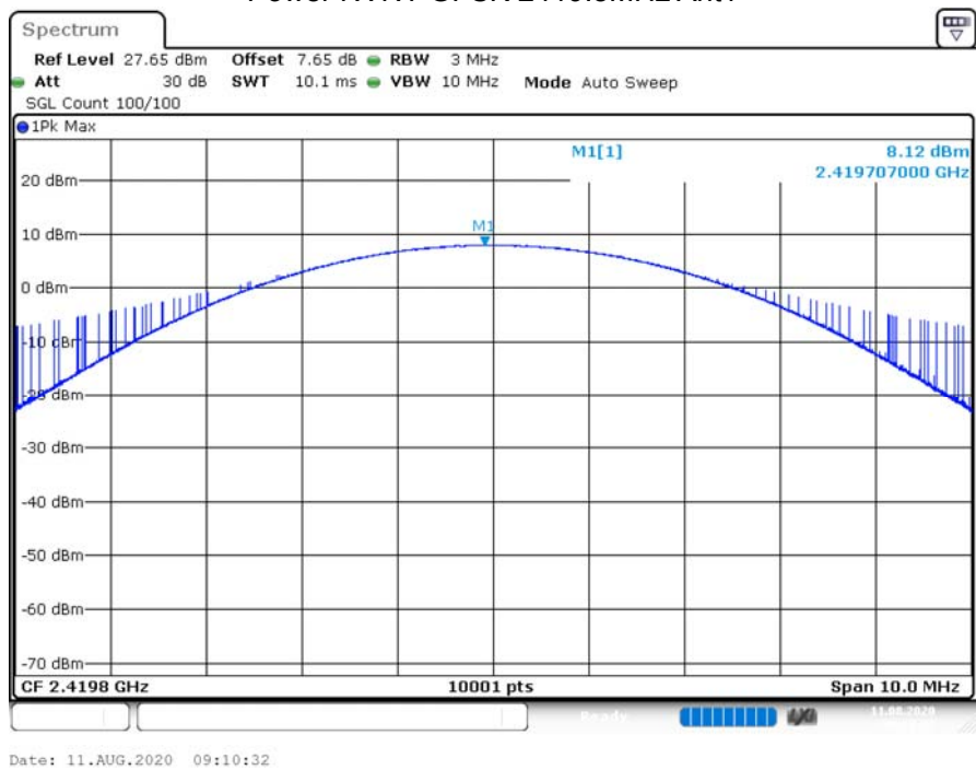
Power NVNT GFSK 2419.8MHz Ant1
