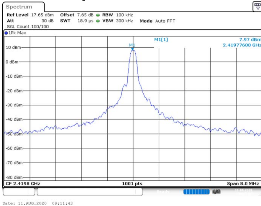
Band Edge NVNT GFSK 2419.8MHz Ant1 Emission
