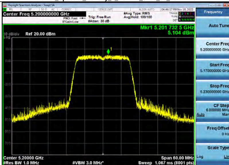
Power Spectral Density 5_2GWiFi_5200_00_20M.PNG
