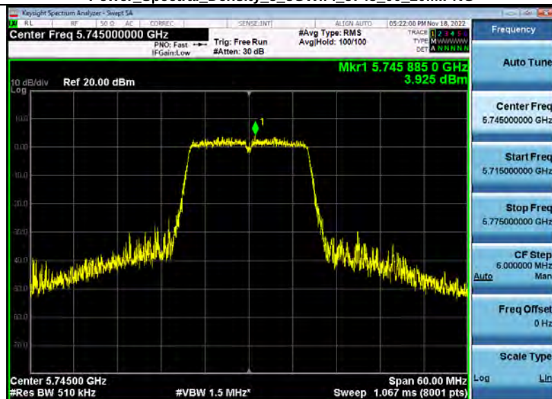
Power_Spectral_Density_5_8GWiFi_5745_00_20M.PNG
