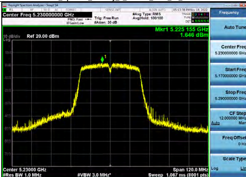
Power Spectral Density 5_2GWiFi_5230_00_40M.PNG
