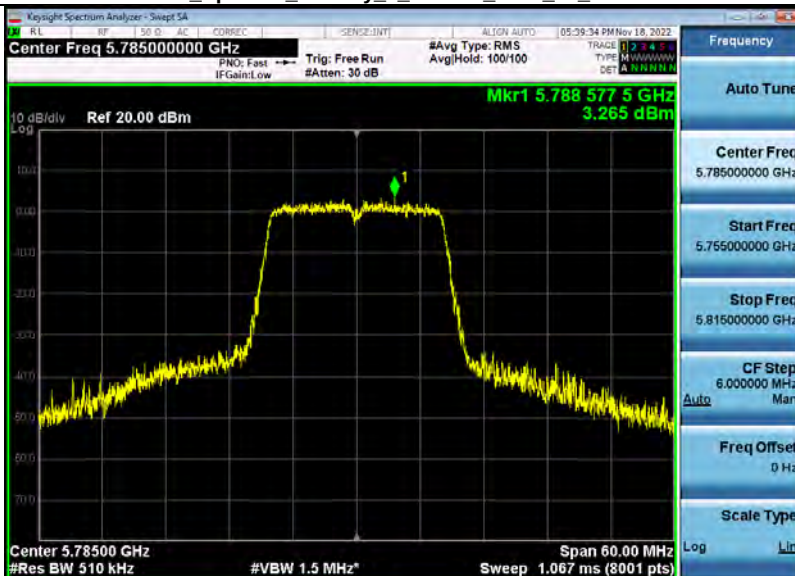
Power Spectral Density 5_8WiFi_5785_00_20M.PNG
