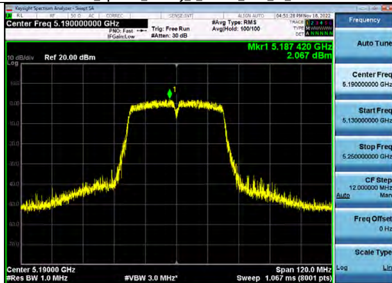
Power Spectral Density 5_2GWiFi_5190_00_40M.PNG
