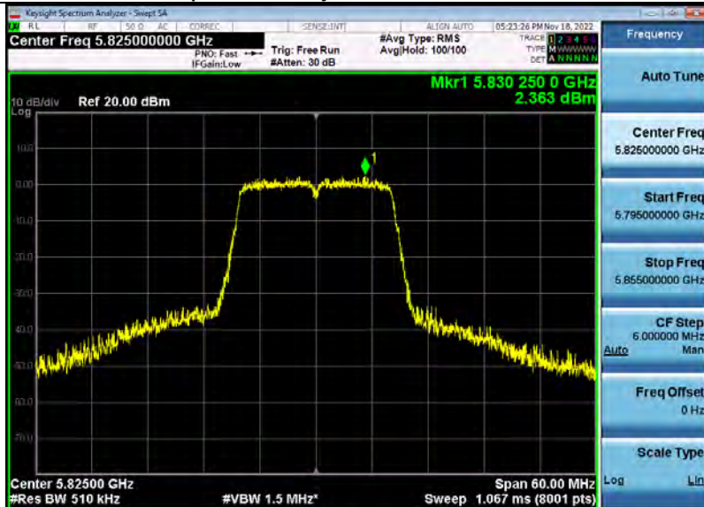
Power Spectral Density 5_8WiFi_5825_00_20M.PNG
