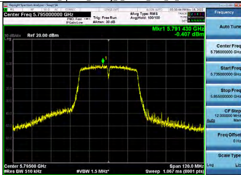
Power Spectral Density 5_8WiFi_5795_00_40M.PNG
