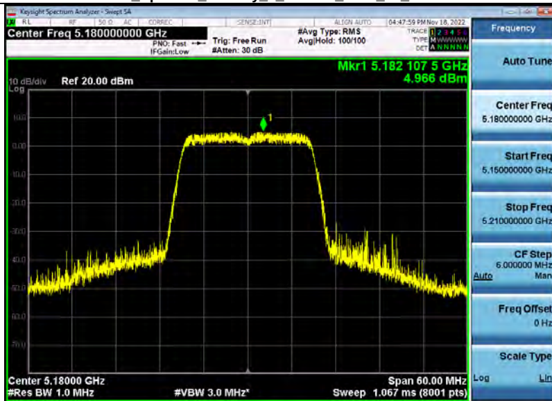
Power Spectral Density 5_2GWiFi_5180_00_20M.PNG
