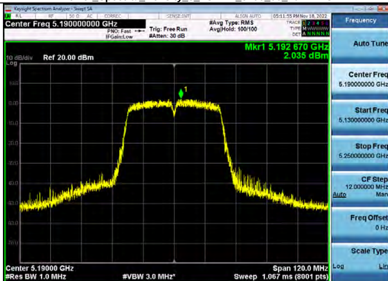
Power Spectral Density 5_2GWiFi_5190_00_40M.PNG
