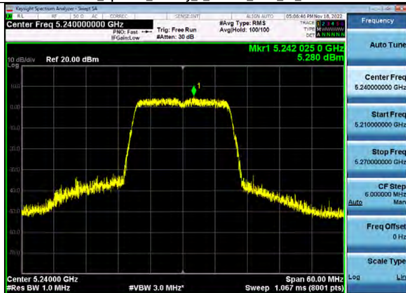
Power Spectral Density 5_2GWiFi_5240_00_20M.PNG
