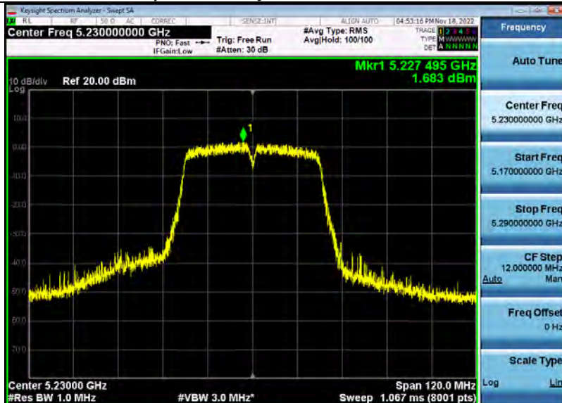
Power Spectral Density 5_2GWiFi_5230_00_40M.PNG
