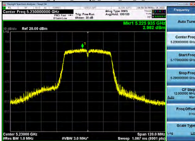
Power_Spectral_Density_5_2GWiFi_5230_00_40M.PNG
