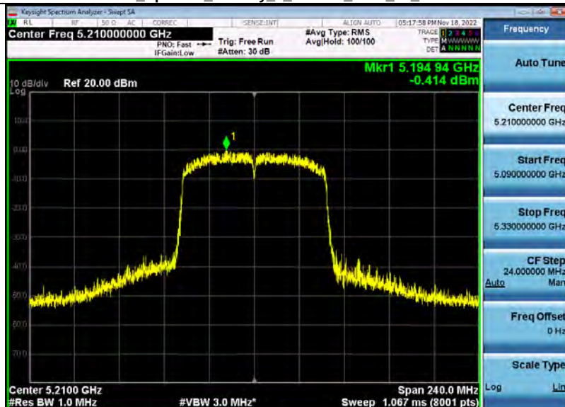
Power Spectral Density 5_2GWiFi_5210_00_80M.PNG
