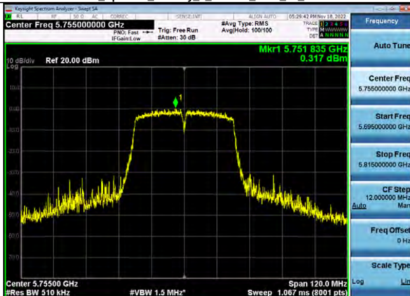
Power Spectral Density 5_8WiFi_5755_00_40M.PNG
