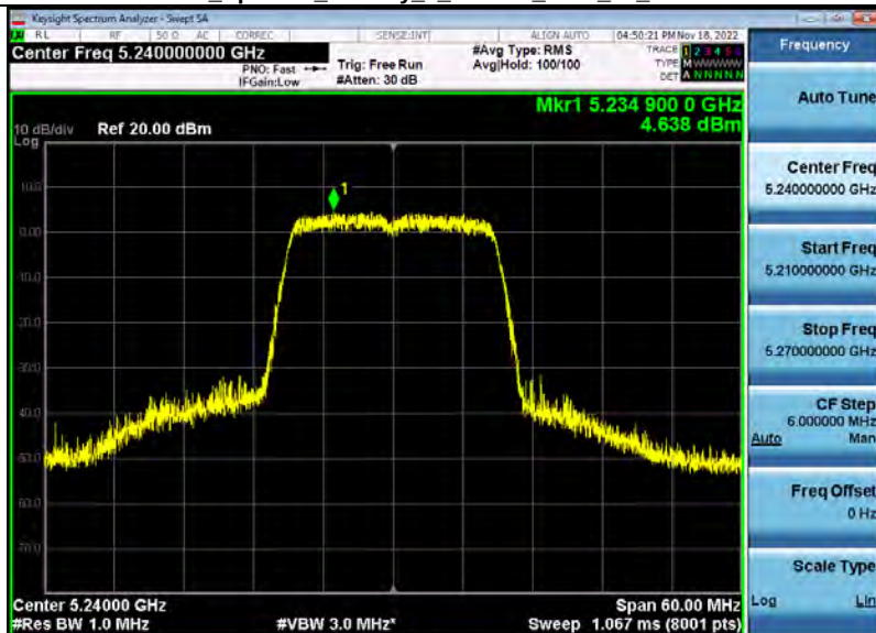
Power Spectral Density 5_2GWiFi_5240_00_20M.PNG
