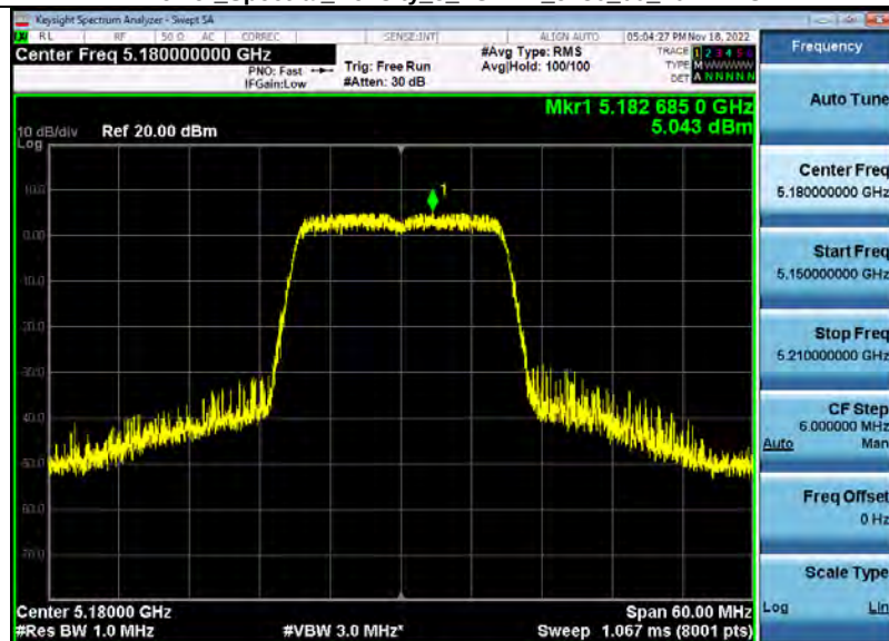
Power Spectral Density 5_2GWiFi_5180_00_20M.PNG
