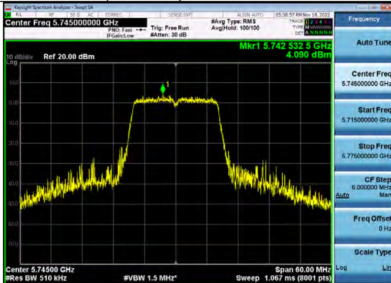
Power Spectral Density 5_8WiFi_5745_00_20M.PNG
