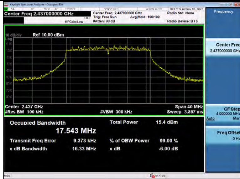
-6dB Bandwidth 2_4GWiFi 2437_00_ANT2
