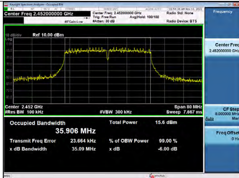
-6dB_Bandwidth_2_4GWiFi_2452_00_ANT2
