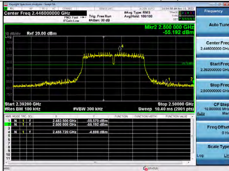
Bandedge_2_4GWiFi_NVNT_ANT1_802_11n(HT40)_2452_00
