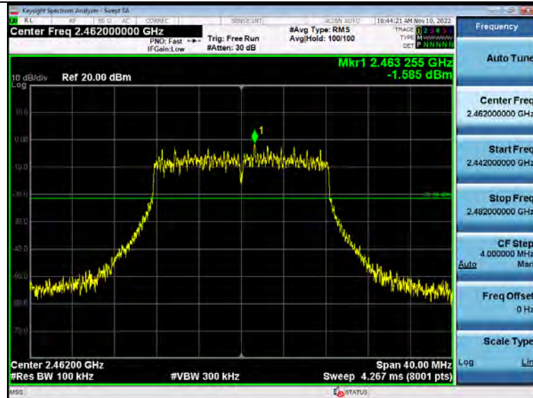
2 Spurious Emission 2 4GWiFi_NVNT_ANT1_802_11g_2462_00
