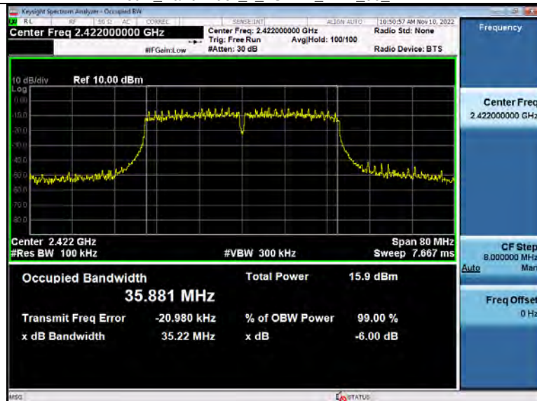
-6dB Bandwidth 2_4GWiFi 2422_00_ANT2
