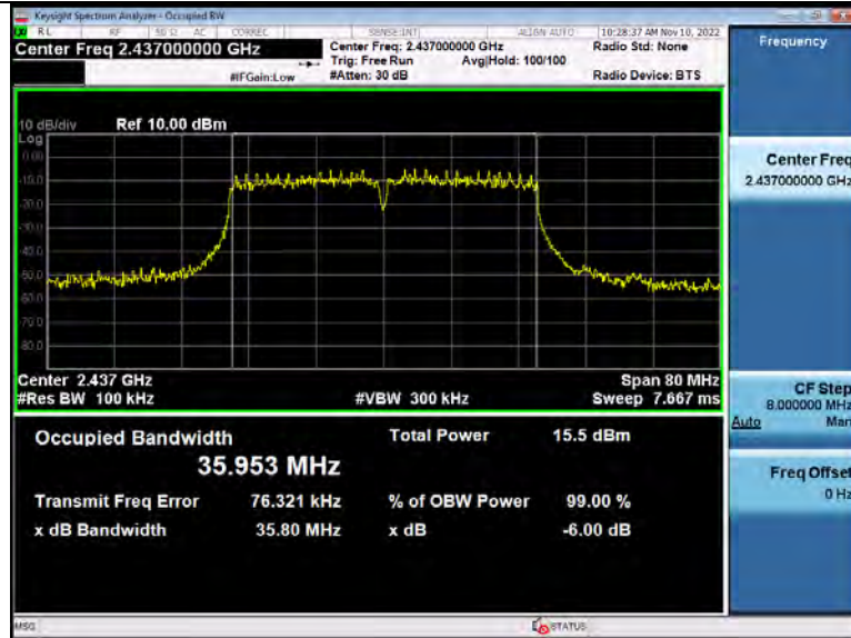
-6dB Bandwidth 2_4GWiFi 2437_00_ANT1
