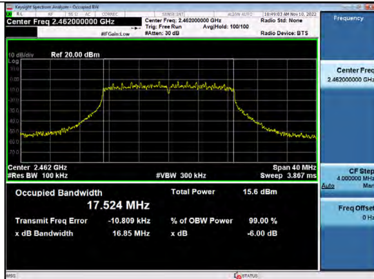
-6dB Bandwidth 2_4GWiFi 2462_00_ANT2
