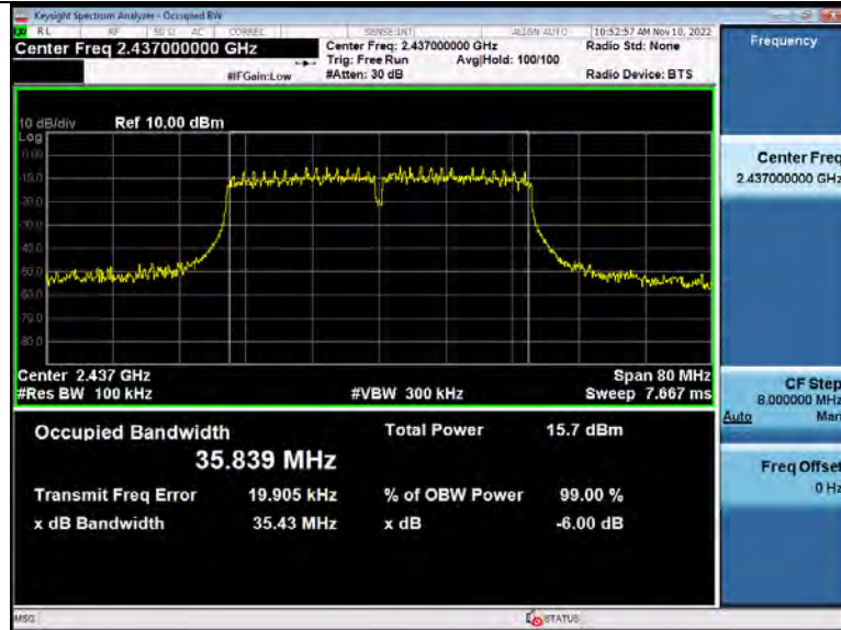
-6dB_Bandwidth_2_4GWiFi_2437_00_ANT2
