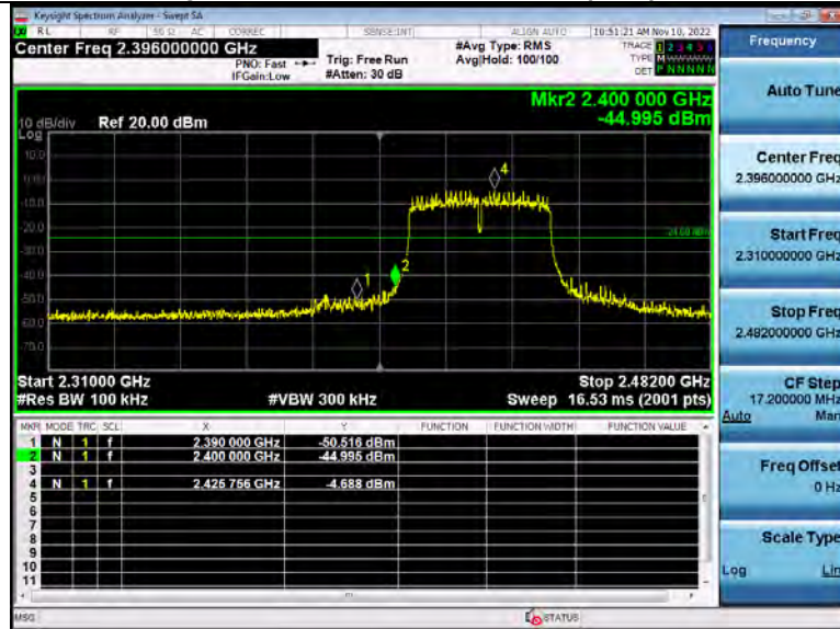
Bandedge_2_4GWiFi_NVNT_ANT1_802_11n(HT40)_2422_00
