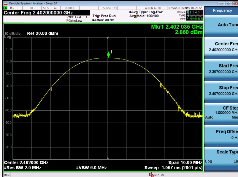
Peak Output Power_BLE_1Mbps_2402
