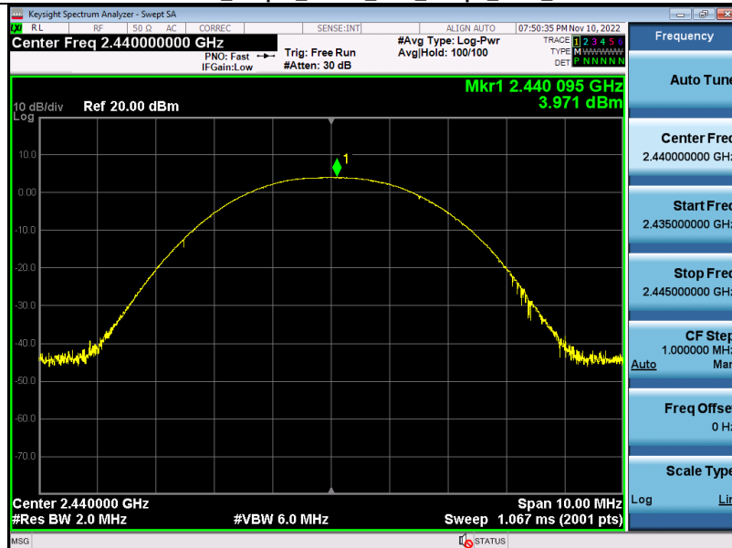
Peak Output Power_BLE_1Mbps_2440_00
