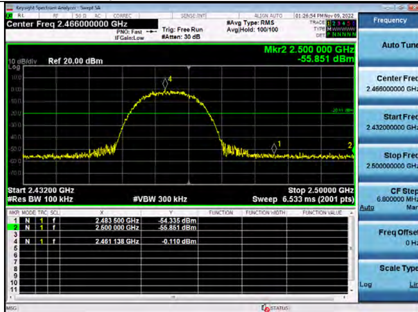
2_Bandedge_2_4GWiFi_NVNT_ANT2_802_11b_2462_00-ANT2
