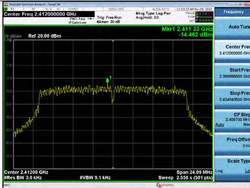
Power Spectral Density_2_4GWiFi_2412_00-ANT1
