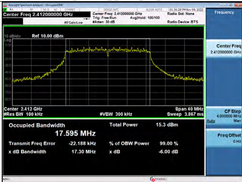
-6dB_Bandwidth_2_4GWiFi_2412_00-ANT2
