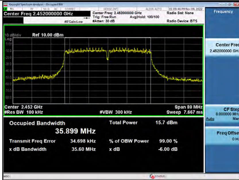
-6dB_Bandwidth_2_4GWiFi_2452_00-ANT1
