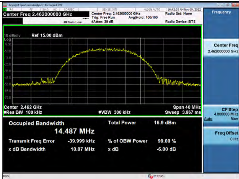
-6dB_Bandwidth_2_4GWiFi_2462_00-ANT1
