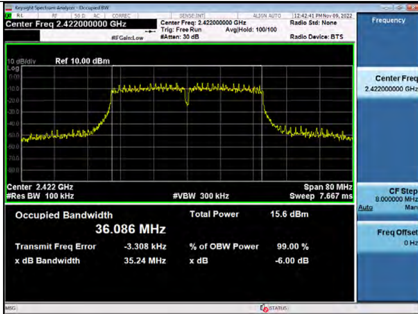
-6dB_Bandwidth_2_4GWiFi_2422_00-ANT1
