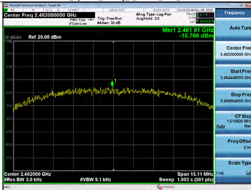
Power_Spectral_Density_2_4GWiFi_2462_00-ANT1
