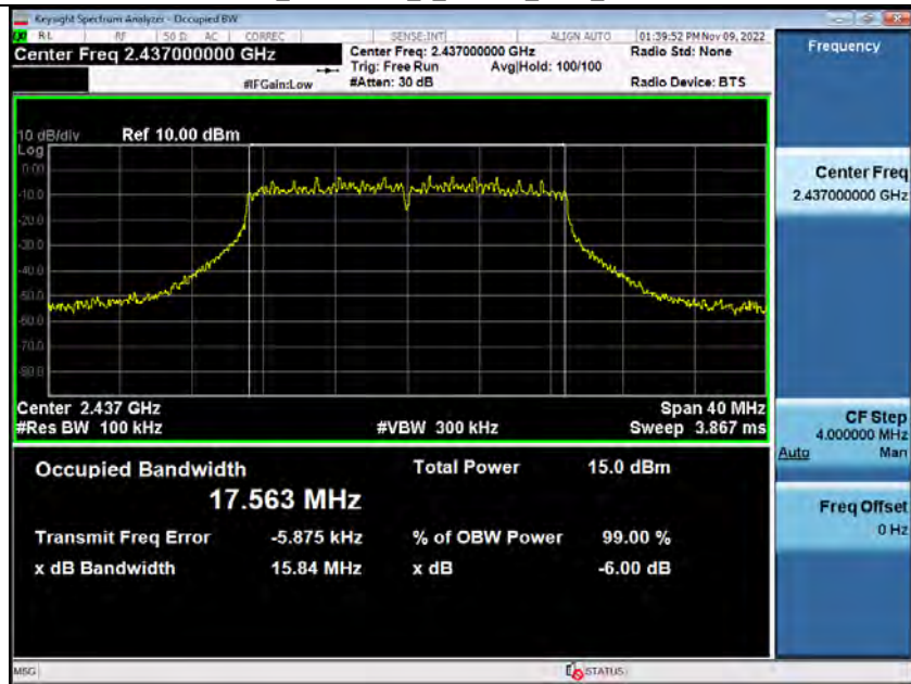
-6dB_Bandwidth_2_4GWiFi_2437_00-ANT2
