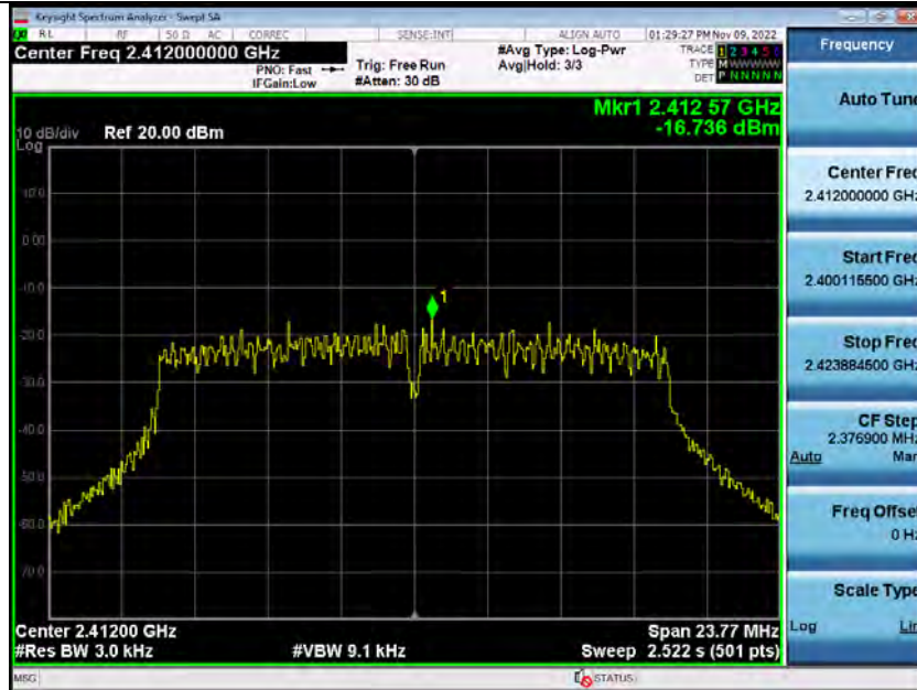
Power Spectral Density_2_4GWiFi_2412_00-ANT2
