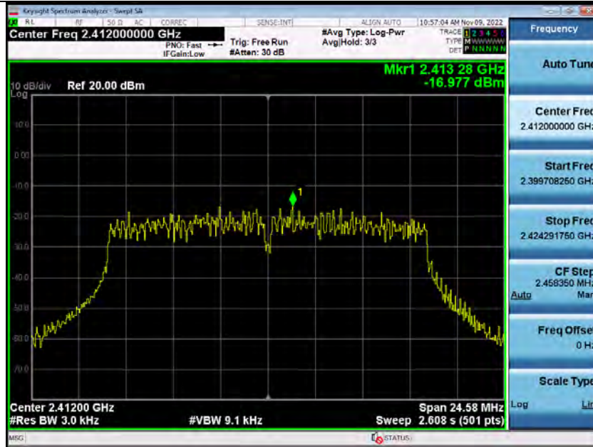
Power_Spectral_Density_2_4GWiFi_2412_00-ANT1
