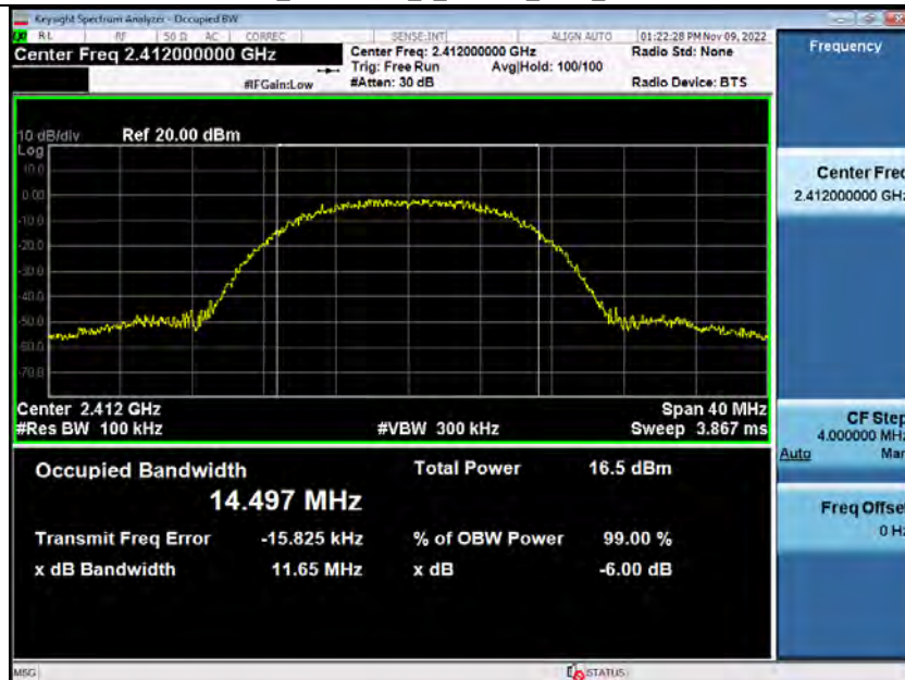
-6dB_Bandwidth_2_4GWiFi_2412_00-ANT2
