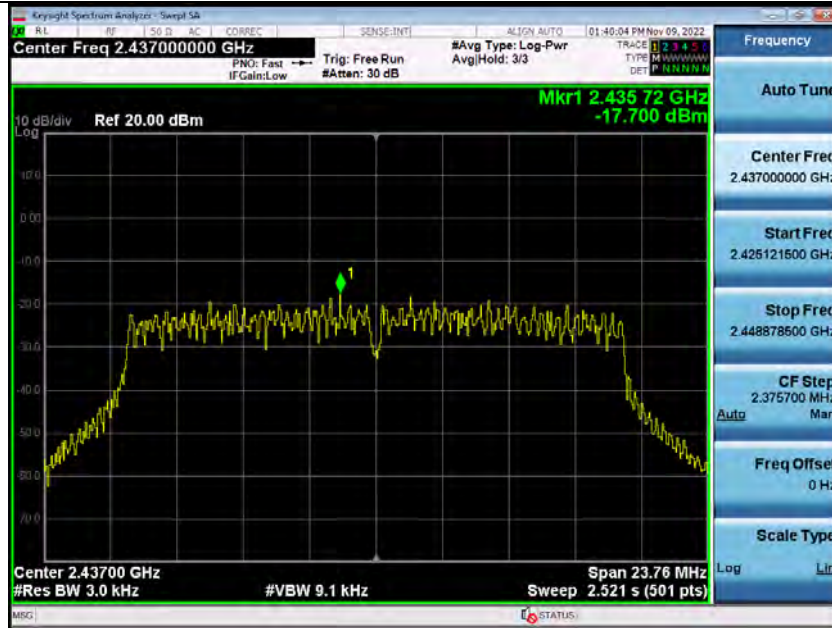
Power_Spectral_Density_2_4GWiFi_2437_00-ANT2
