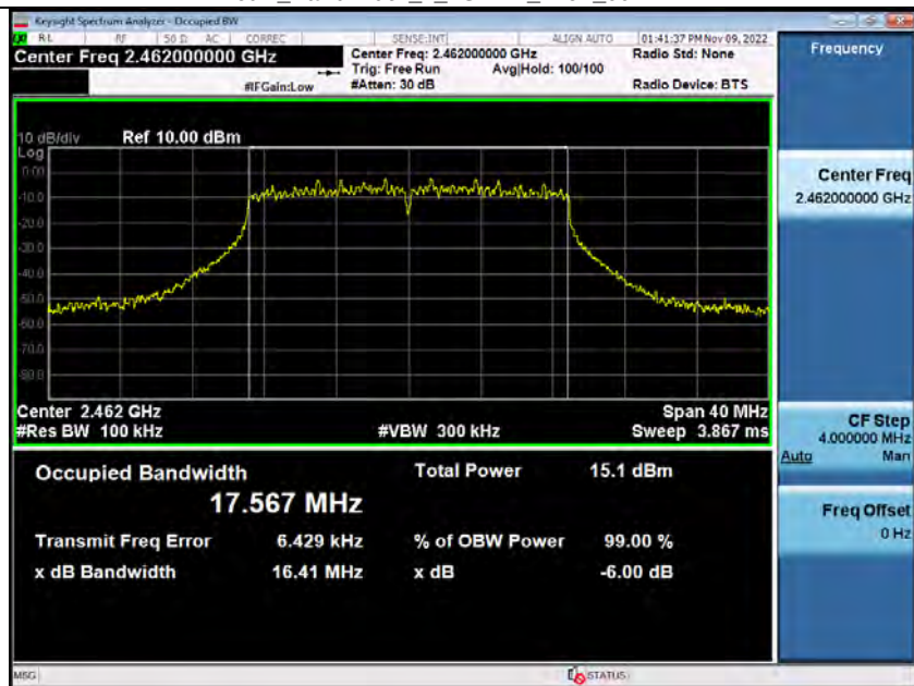
-6dB_Bandwidth_2_4GWiFi_2462_00-ANT2
