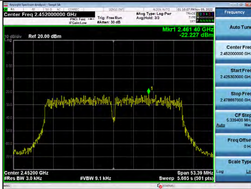
Power Spectral Density_2_4GWiFi_2452_00-ANT1
