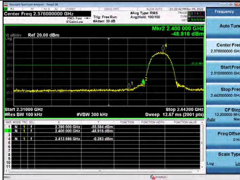
2_Bandedge_2_4GWiFi_NVNT_ANT2_802_11b_2412_00-ANT2
