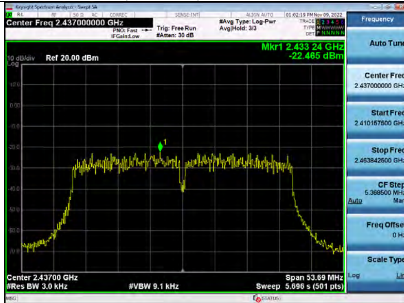
Power Spectral Density_2_4GWiFi_2437_00-ANT1
