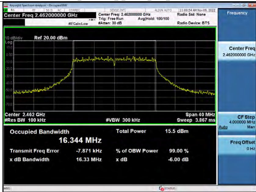
-6dB_Bandwidth_2_4GWiFi_2462_00-ANT1
