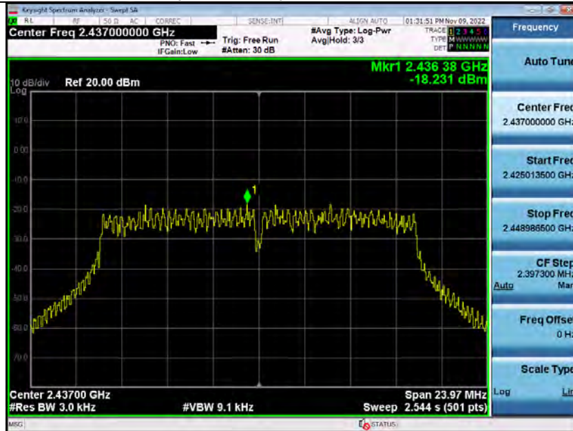
Power Spectral Density_2_4GWiFi_2437_00-ANT2
