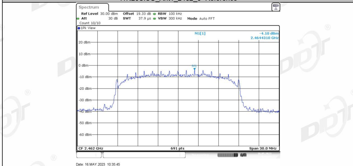
11N20SISO Ant1 2462 30~1000
