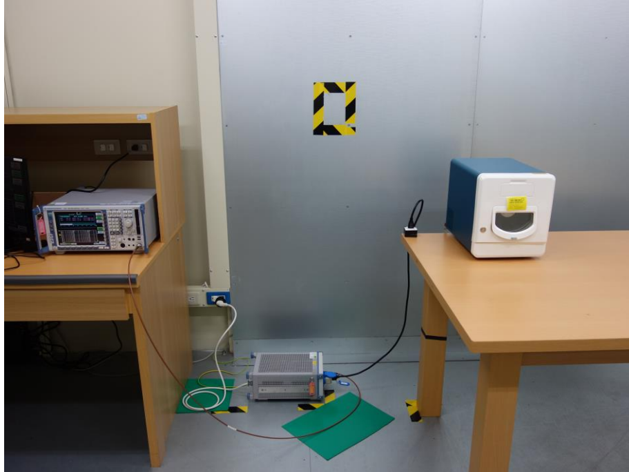
Photograph 7: Test Setup for Mains Conducted Emissions (Front View)
