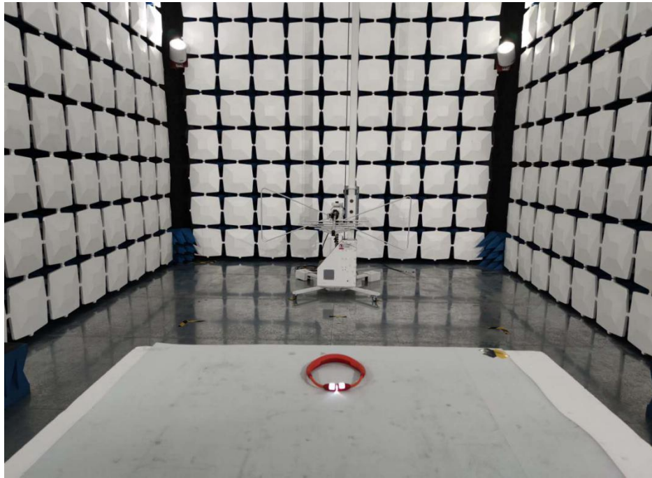
Below 1GHz for radiated emission test setup
