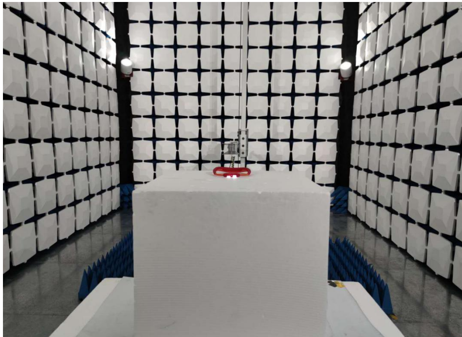
Above 1GHz for radiated emission test setup
