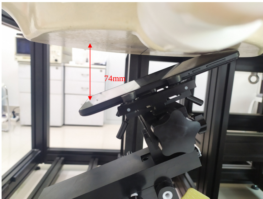
Head Flat Setup Photo (71mm)
