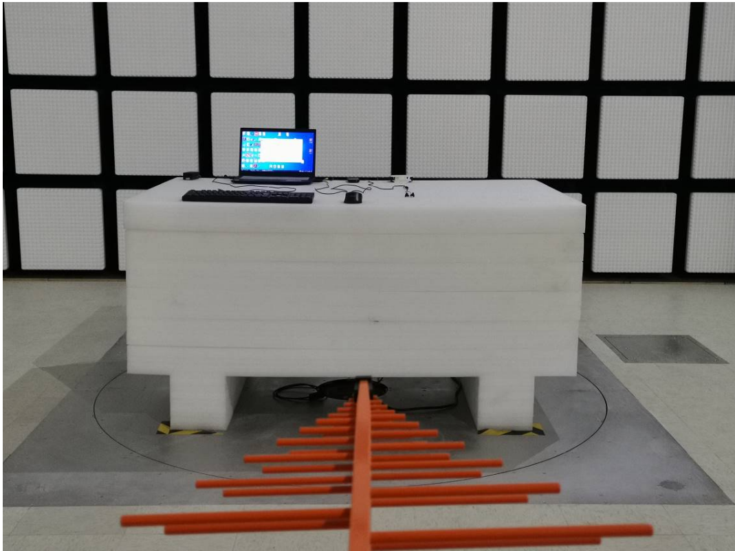
Radiated Emission Below 1G rear View
