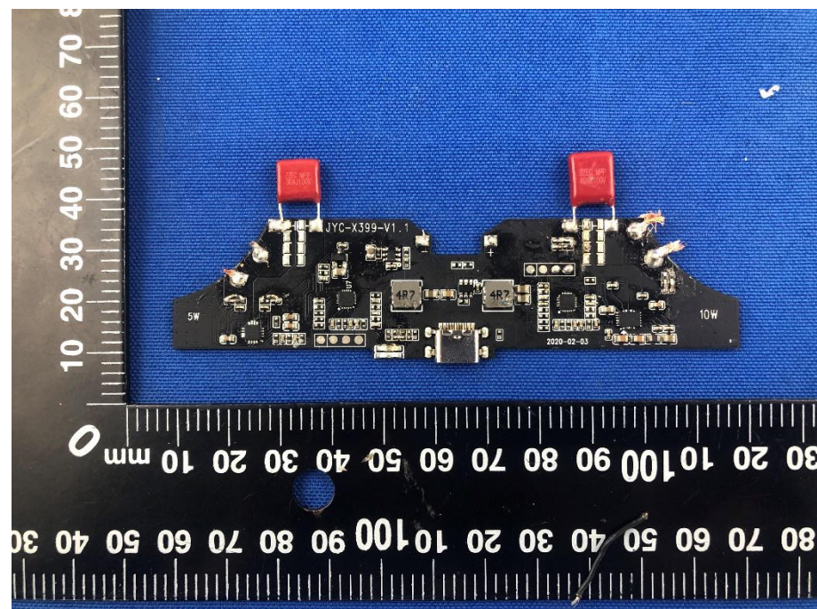
SECOND BOARD TOP VIEW
