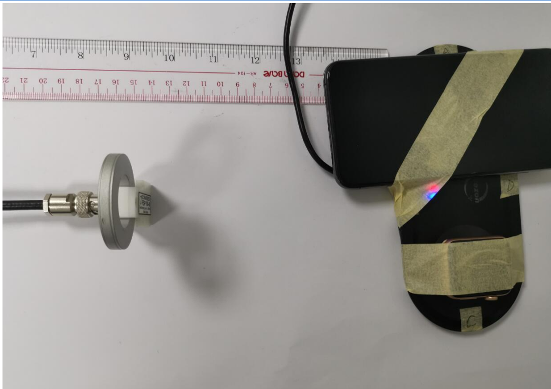
H-field Test Setup Photo of Position B(15cm)
