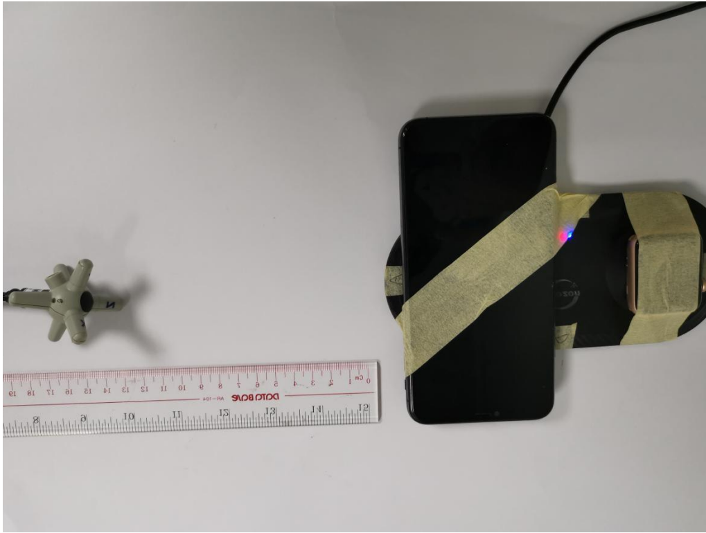
E-field Test Setup Photo of Position A(15cm)
