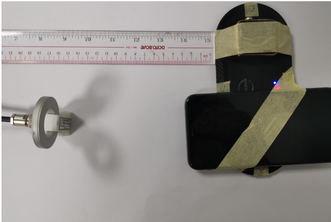
H-field Test Setup Photo of Position D(15cm)
