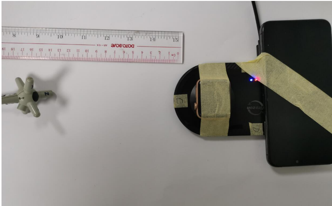
E-field Test Setup Photo of Position C(15cm)
