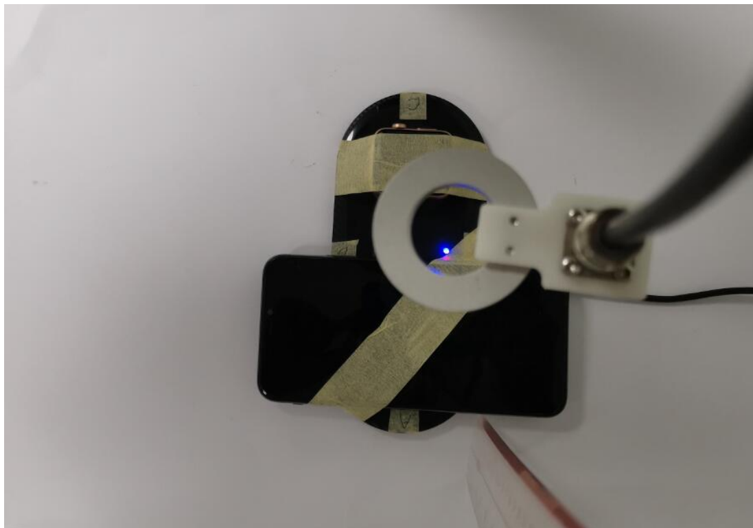
H-field Test Setup Photo of Position E(20cm)
