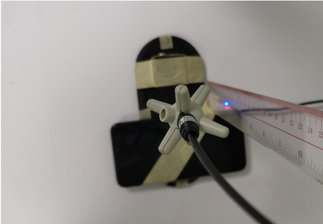
E-field Test Setup Photo of Position E(20cm)
