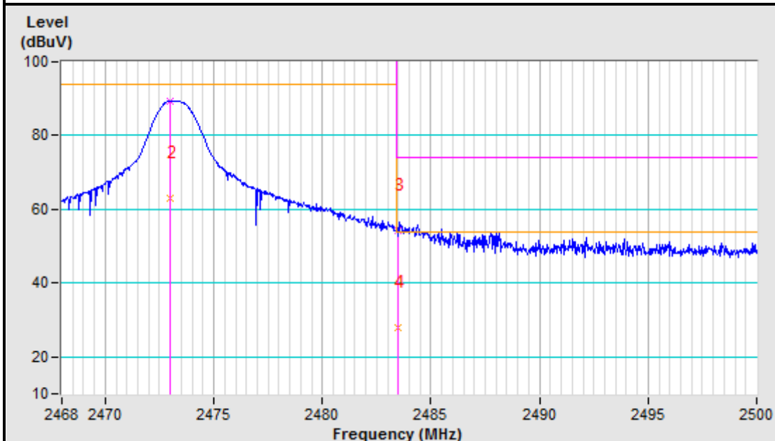
2473MHz Vertical
