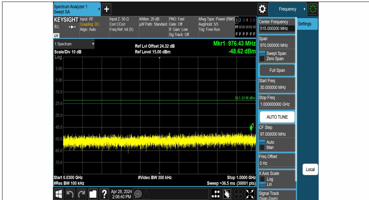
BLE_1M-Ant1-2440-30~1000-PASS
