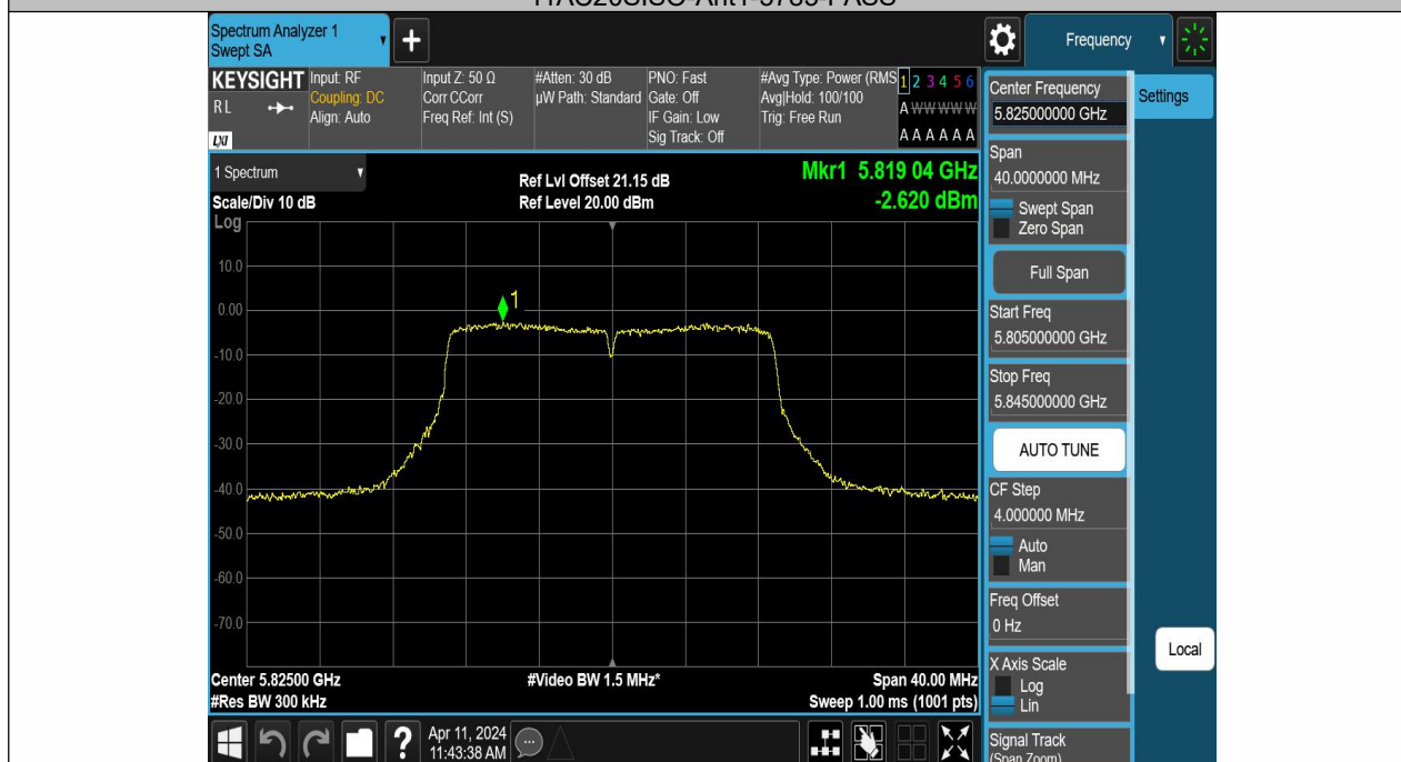
11AC20SISO-Ant1-5825-PASS
