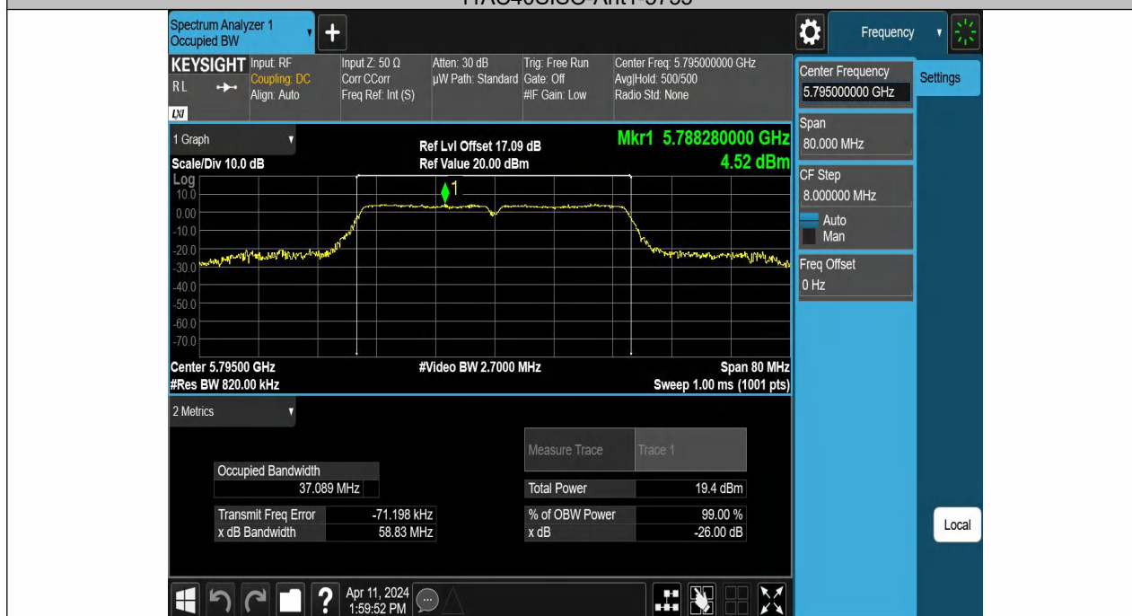
11AC40SISO-Ant1-5795
