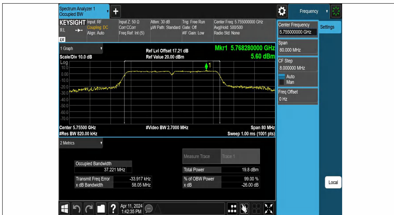
11AC40SISO-Ant1-5755
