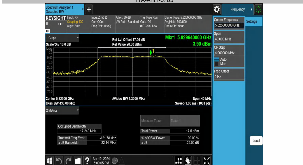
11A-Ant1-5825
