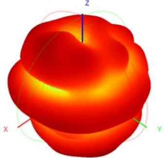
5350.0MHz H+V, Eff: 28.5%
