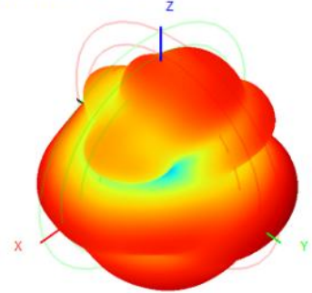
2500.0MHz H+V, Eff: 54.8%
