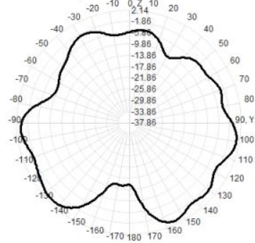
5150.0MHz Total(E2-YZ), Max= -2.09dBi
