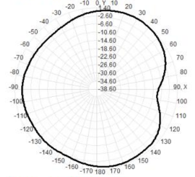
Total(H+V), Max= 2.14dBi, CirD=10.82
