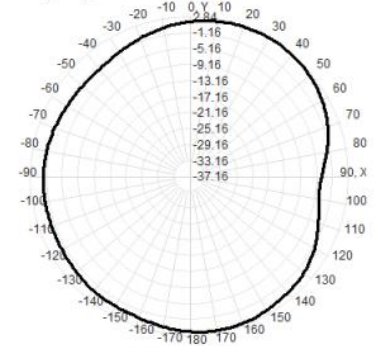
Total(H+V), Max= 1.40dBi, CirD=10.19
