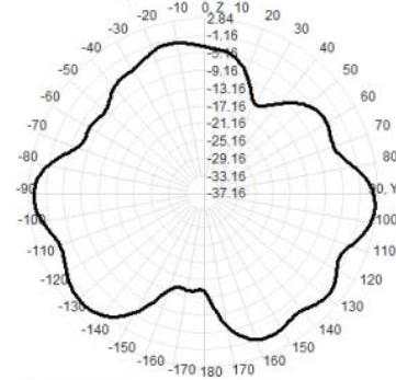
2450.0MHz Total(E2-YZ), Max= 0.73dBi
