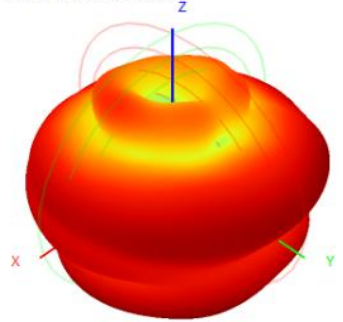
5350.0MHz H+V, Eff: 28.5%
