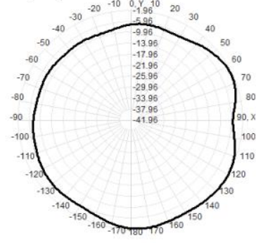
Total(H+V), Max= -1.96dBi, CirD=6.94
