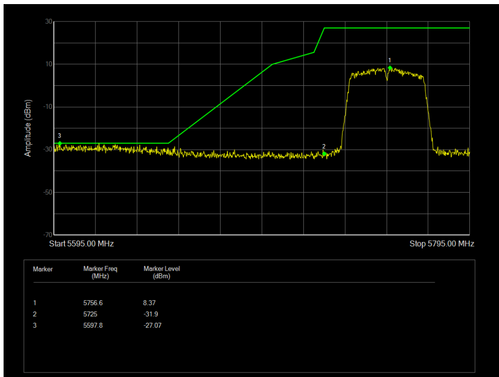
Band Edge NVNT 802.11ac40 5755MHz Low Ant 4
