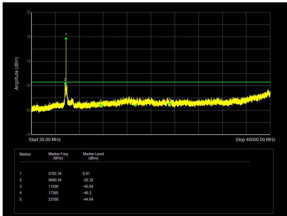
Tx. Spurious NVNT 802.11n(HT40) 5755MHz Ant 4 Emission
