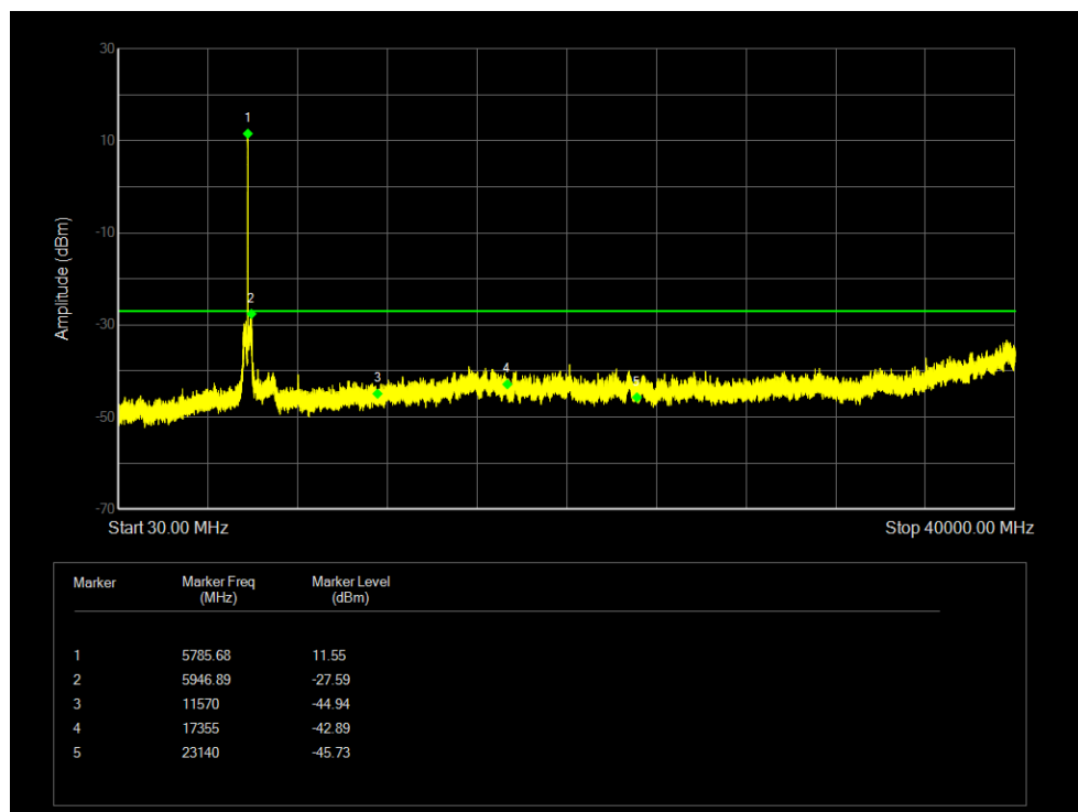
Tx. Spurious NVNT 802.11a 5785MHz Ant 4 Emission
