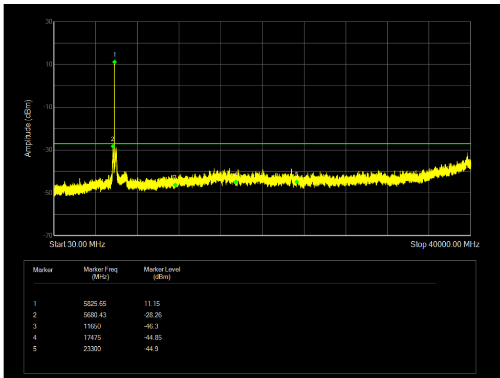
Tx. Spurious NVNT 802.11ac20 5825MHz Ant 3 Emission
