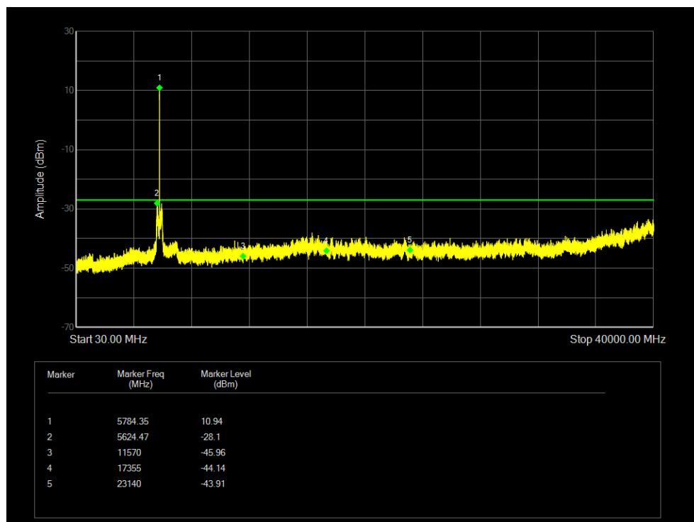
Tx. Spurious NVNT 802.11ac20 5785MHz Ant 4 Emission
