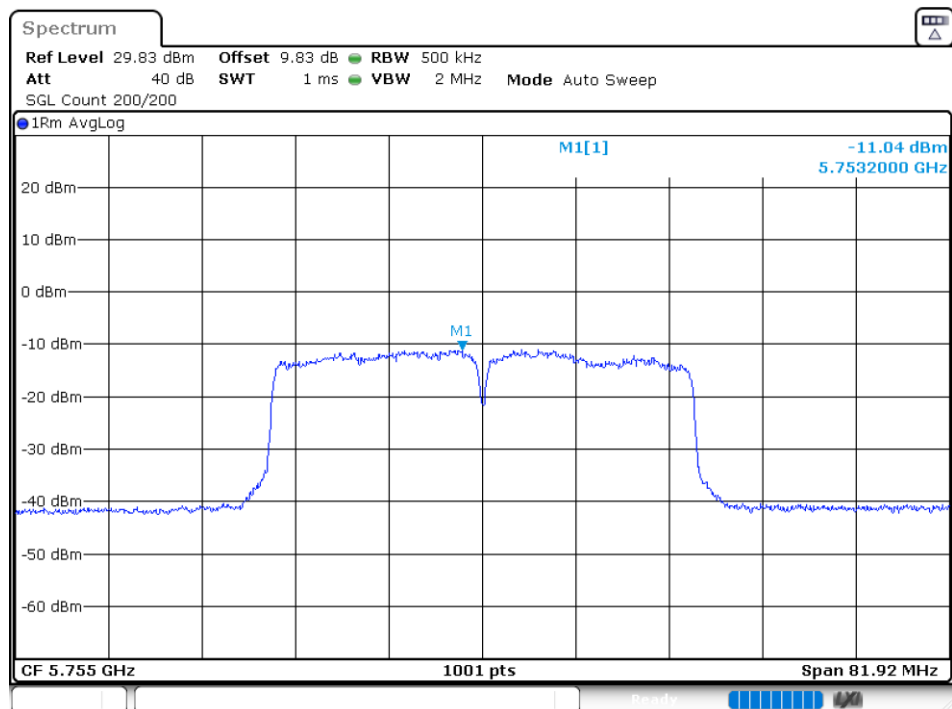
PSD NVNT 802.11ac40 5755MHz Ant 4
