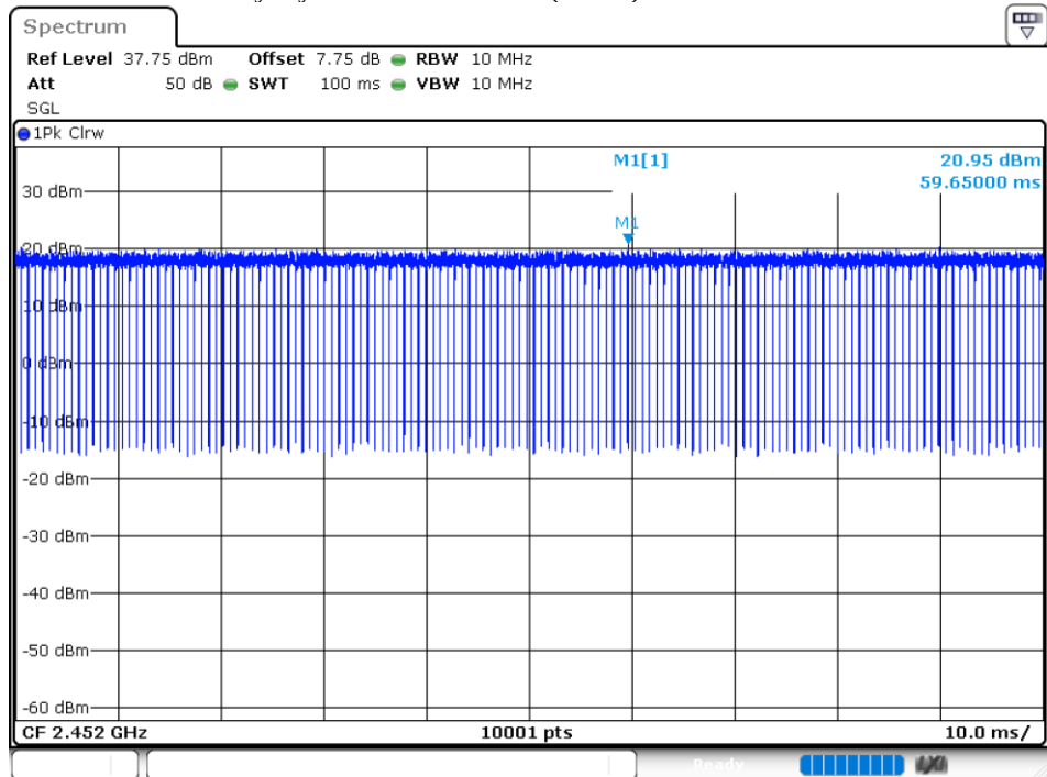
Duty Cycle NVNT 802.11n(HT40) 2452MHz Ant 4
