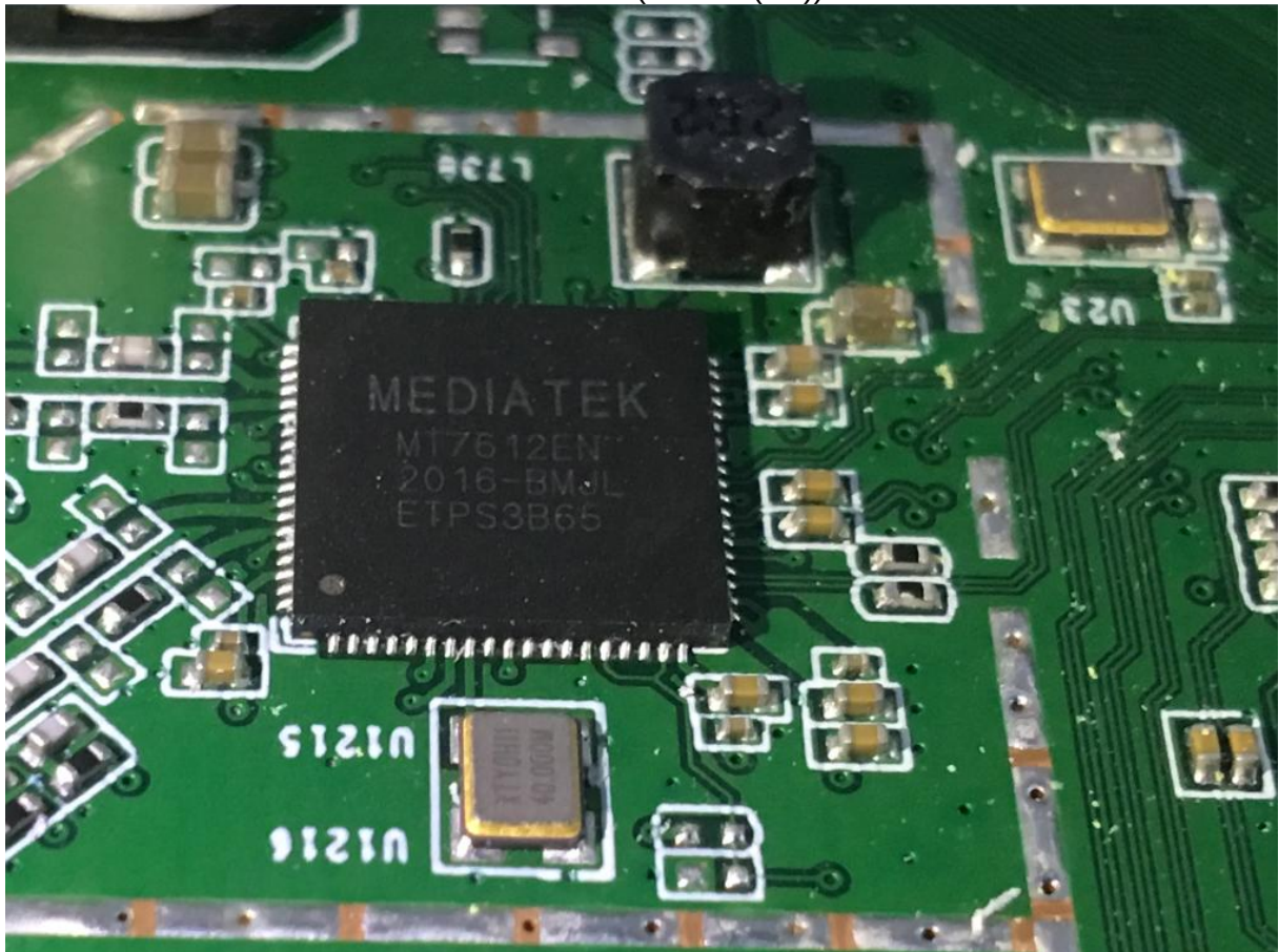
Photo28 (Wi-Fi 1 (5G))
