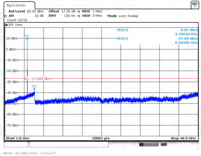
11AC20-CDD-Ant1-5500-1000~40000-PASS
