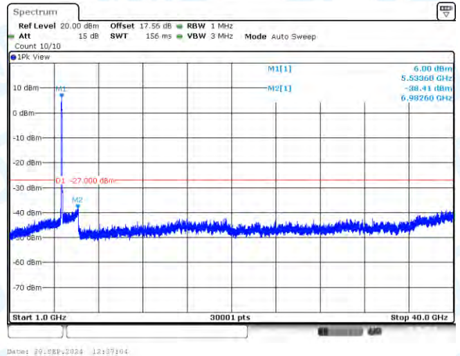
11AC80-CDD-Ant1-5530-1000~40000-PASS
