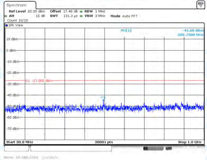
11AC40-CDD-Ant2-5190-30~1000-PASS
