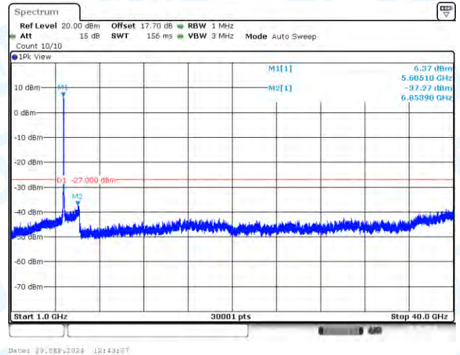
11AC80-CDD-Ant1-5610-1000~40000-PASS
