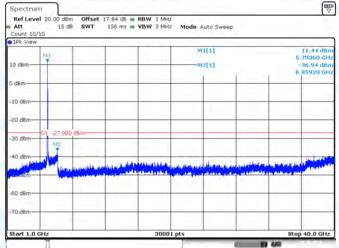
11AC40-CDD-Ant1-5795-1000~40000-PASS
