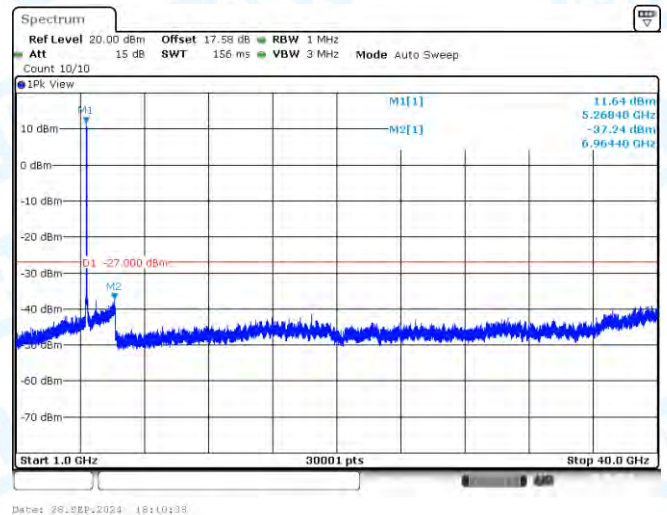
11N40-CDD-Ant3-5270-1000~40000-PASS
