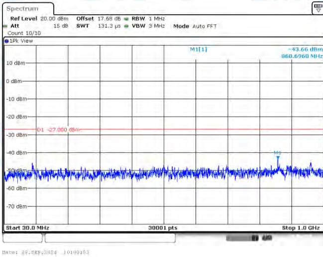
11AC40-CDD-Ant3-5510-30~1000-PASS
