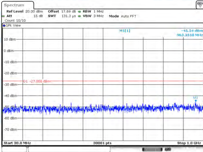
11AC40-CDD-Ant1-5795-30~1000-PASS
