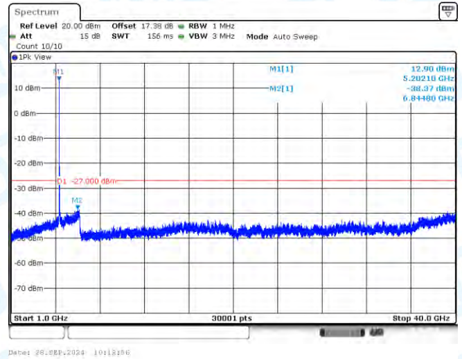
11AC20-CDD-Ant1-5200-1000~40000-PASS
