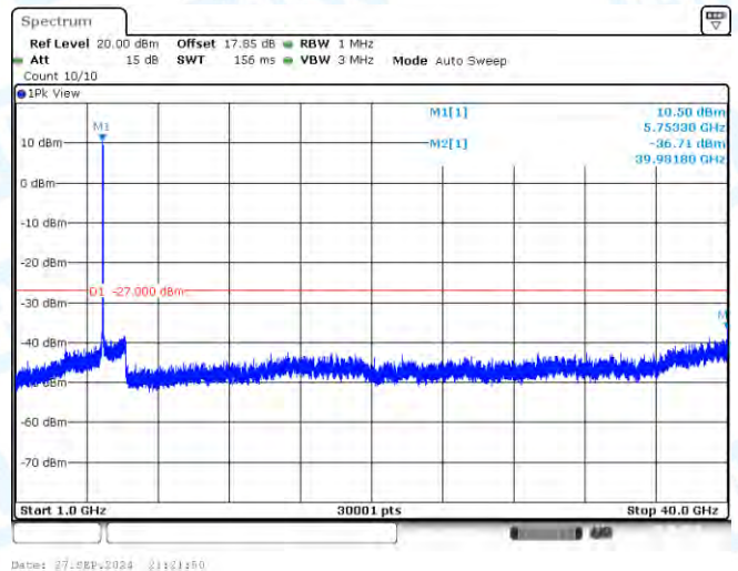
11N40-CDD-Ant3-5755-1000~40000-PASS
