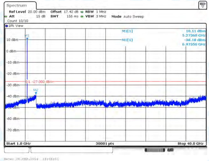
11N40-CDD-Ant1-5270-1000~40000-PASS
