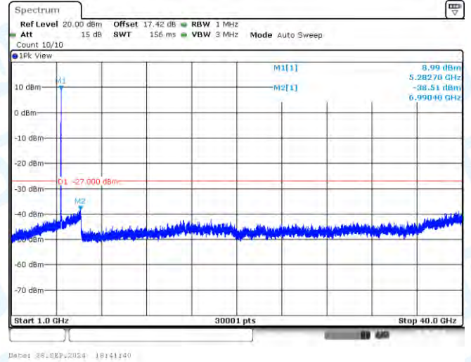
11AC20-CDD-Ant1-5280-1000~40000-PASS
