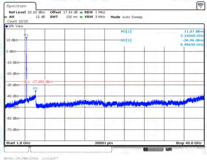
11AC40-CDD-Ant3-5190-1000~40000-PASS
