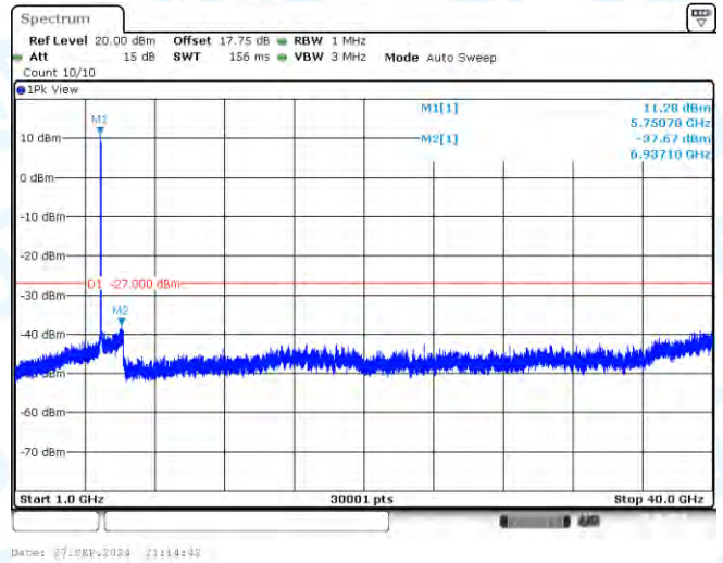
11N40-CDD-Ant1-5755-1000~40000-PASS
