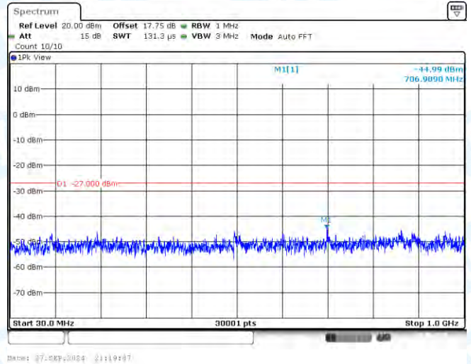
11N40-CDD-Ant2-5755-30~1000-PASS
