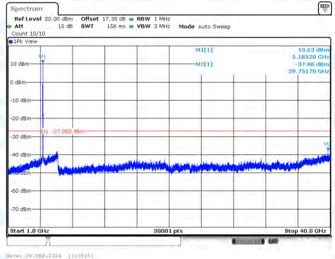
11AC40-CDD-Ant1-5190-1000~40000-PASS
