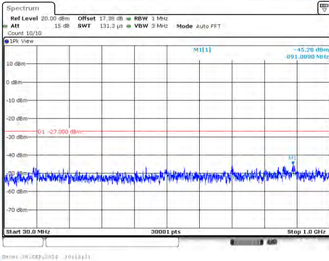
11AC20-CDD-Ant1-5200-30~1000-PASS
