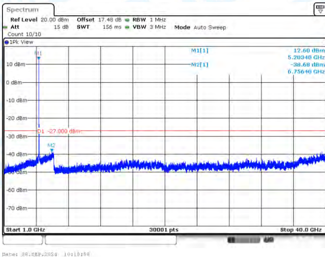
11AC20-CDD-Ant2-5200-1000~40000-PASS
