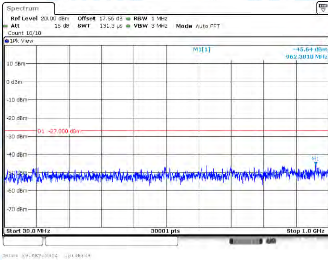
11AC80-CDD-Ant1-5530-30~1000-PASS
