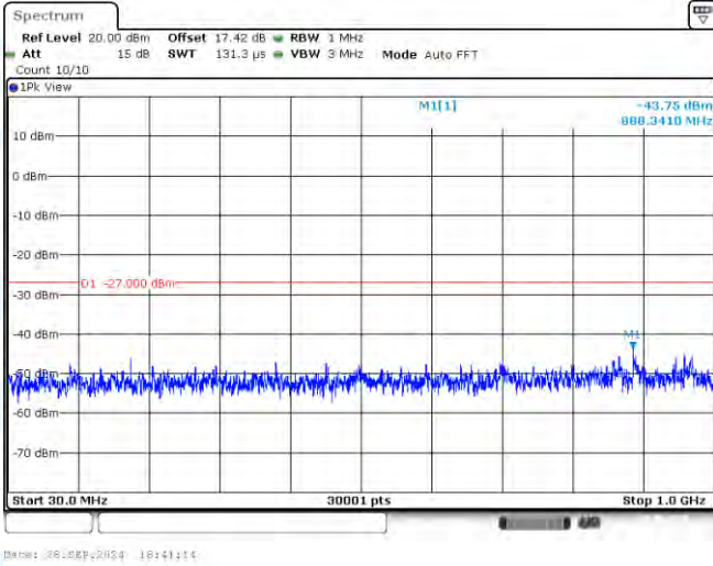
11AC20-CDD-Ant1-5280-30~1000-PASS
