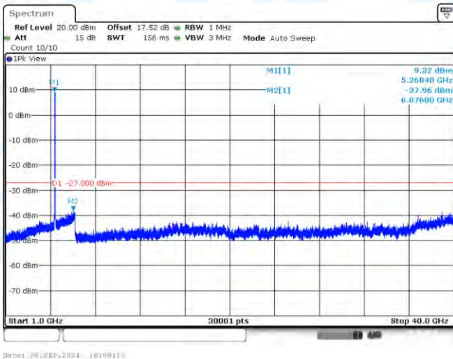
11N40-CDD-Ant2-5270-1000~40000-PASS
