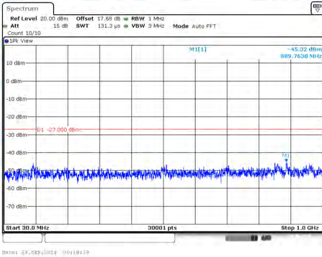
11AC20-CDD-Ant3-5500-30~1000-PASS
