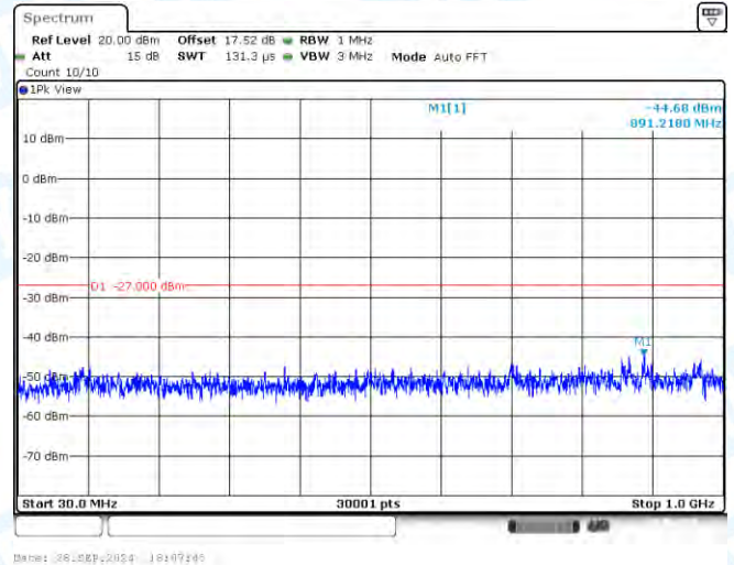
11N40-CDD-Ant2-5270-30~1000-PASS
