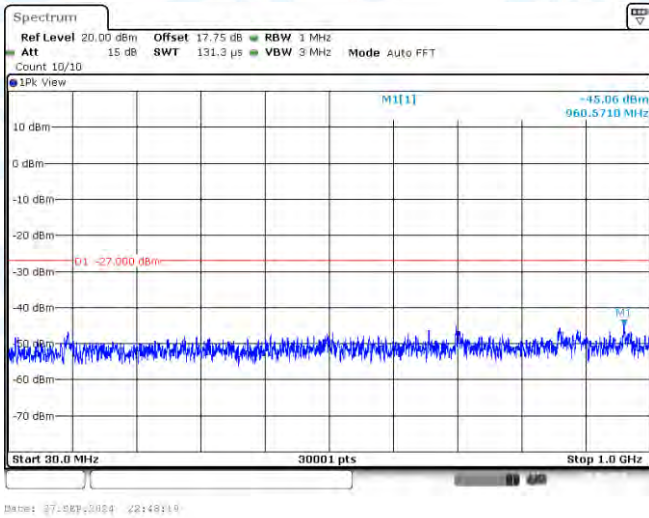
11AC20-CDD-Ant2-5745-30~1000-PASS
