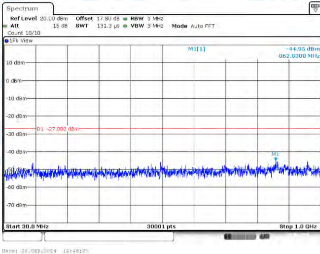
11AC80-CDD-Ant3-5610-30~1000-PASS
