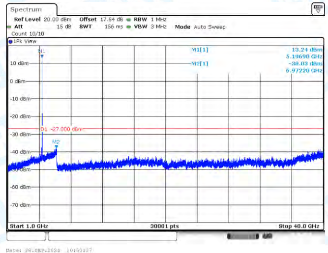
11AC20-CDD-Ant3-5200-1000~40000-PASS
