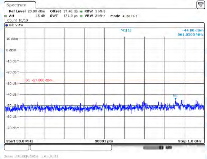
11AC20-CDD-Ant2-5200-30~1000-PASS
