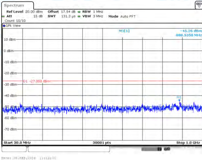
11AC40-CDD-Ant3-5190-30~1000-PASS
