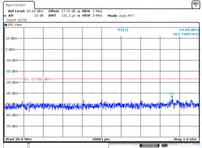
11AC40-CDD-Ant2-5795-30~1000-PASS
