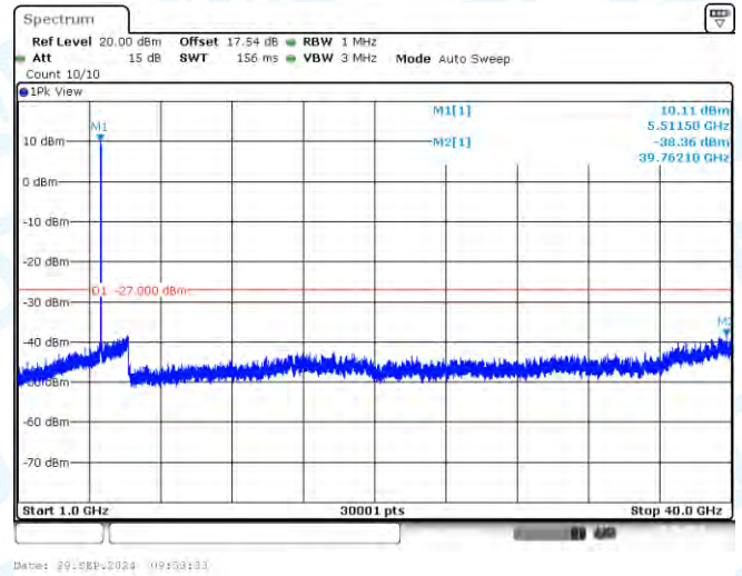
11AC40-CDD-Ant1-5510-1000~40000-PASS
