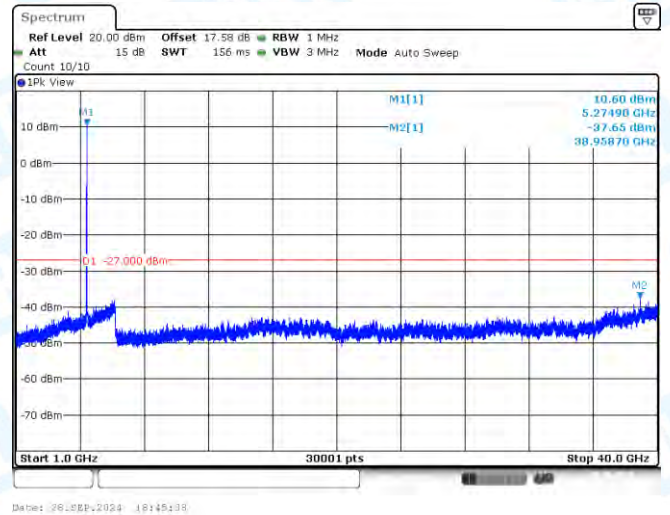
11AC20-CDD-Ant3-5280-1000~40000-PASS
