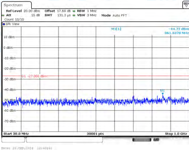
11AC80-CDD-Ant3-5530-30~1000-PASS
