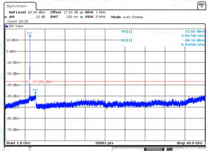
11AC20-CDD-Ant1-5825-1000~40000-PASS
