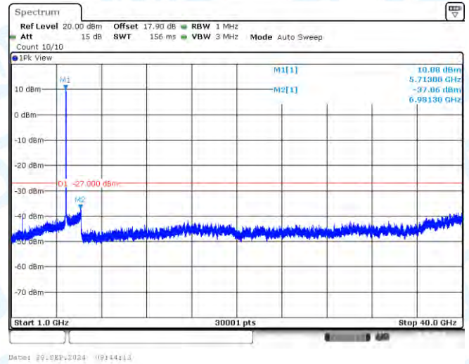
11N40-CDD-Ant1-5710-1000~40000-PASS
