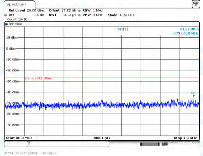
11AC20-CDD-Ant2-5280-30~1000-PASS
