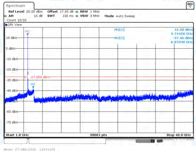
11AC20-CDD-Ant3-5745-1000~40000-PASS
