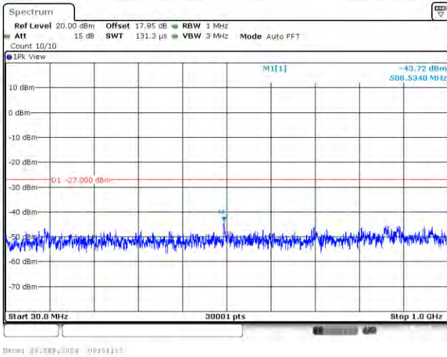
11N40-CDD-Ant3-5710-30~1000-PASS
