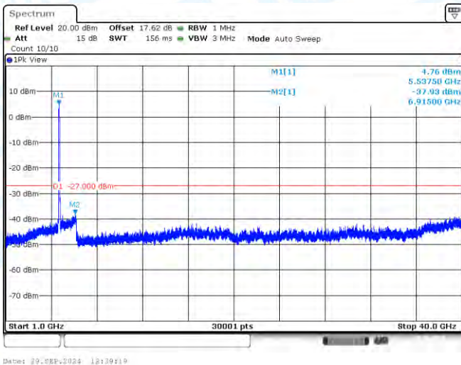
11AC80-CDD-Ant2-5530-1000~40000-PASS
