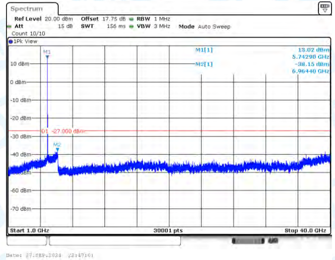
11AC20-CDD-Ant1-5745-1000~40000-PASS
