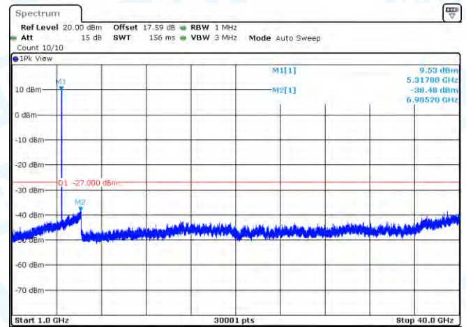
11AC20-CDD-Ant1-5320-1000~40000-PASS
