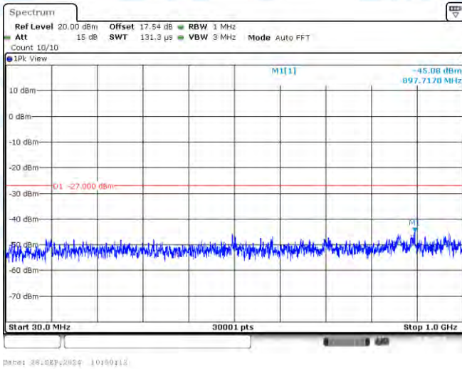
11AC20-CDD-Ant3-5200-30~1000-PASS
