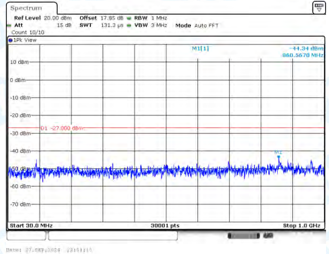
11AC20-CDD-Ant3-5745-30~1000-PASS
