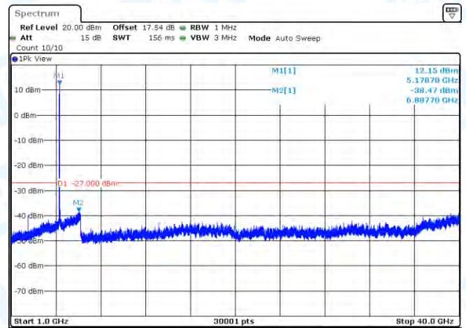
11AC20-CDD-Ant1-5180-1000~40000-PASS
