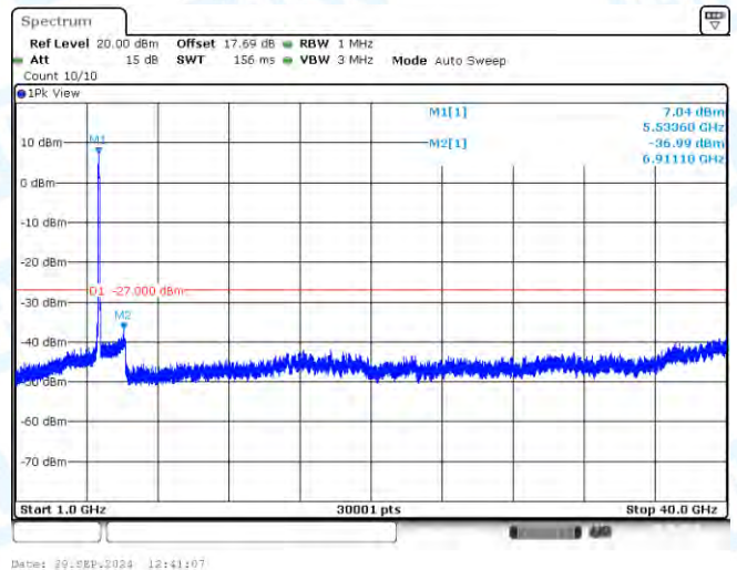
11AC80-CDD-Ant3-5530-1000~40000-PASS
