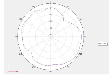
Theta =90 freq=5550MHz
