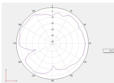
Phi =90 freq=5150MHz
