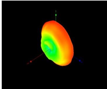
Phi =90 freq=5850MHz
