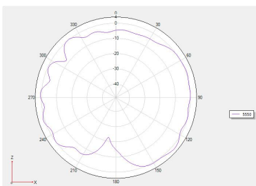
Phi =0 freq=5550MHz
