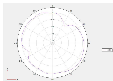
Theta =90 freq=5150MHz
