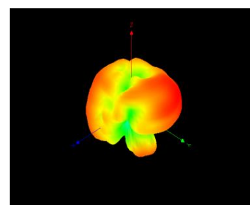
Theta =90 freq=5550MHz
