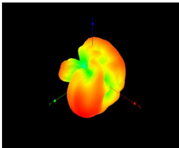
Phi =0 freq=5550MHz
