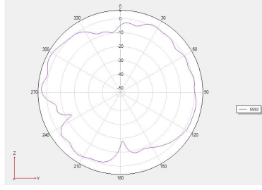
Phi =90 freq=5550MHz
