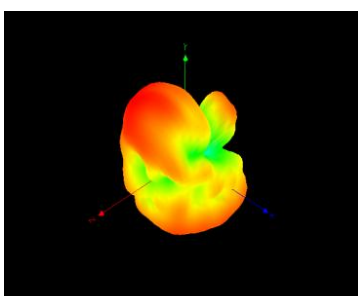
Phi =90 freq=5550MHz
