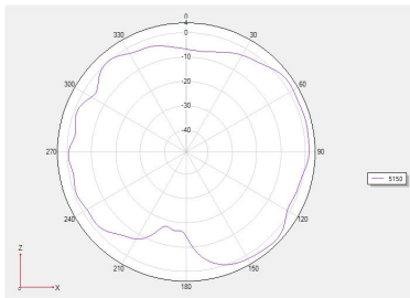
Phi =0 freq=5150MHz
