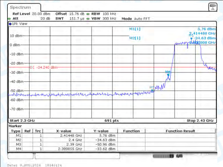
11G-Ant2-2412-PASS
