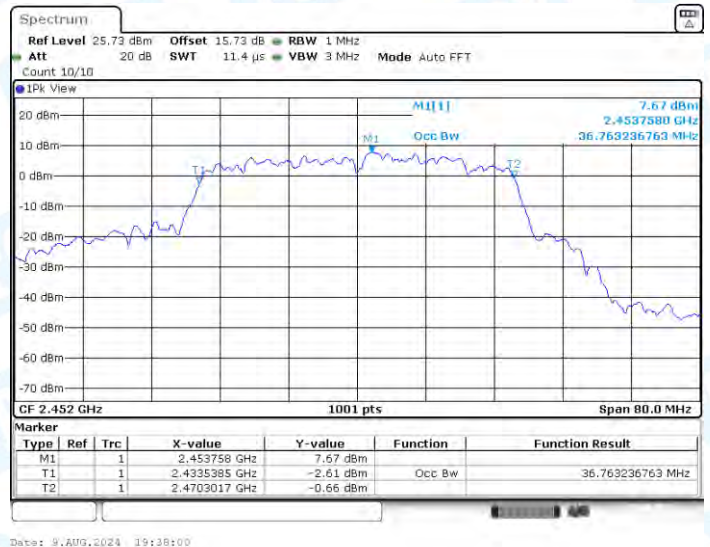
11N40-CDD-Ant2-2452
