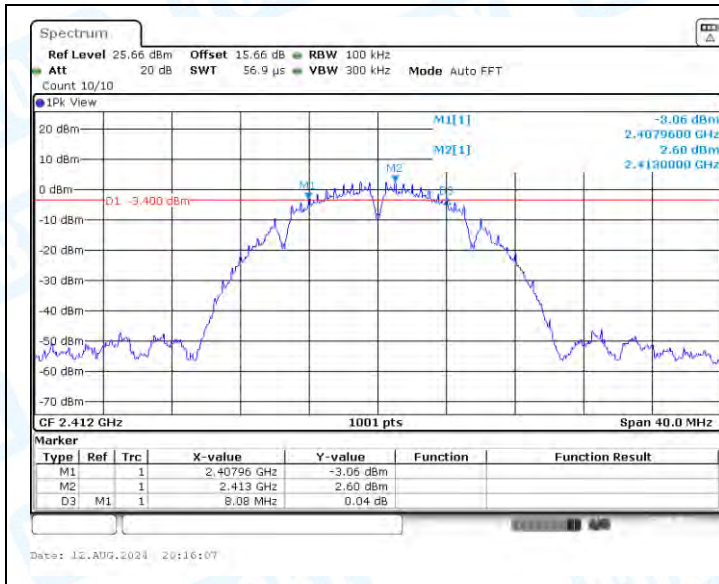
11B-Ant1-2412-PASS
