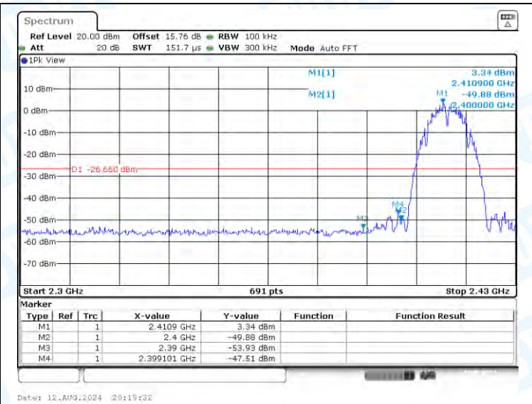
11B-Ant2-2412-PASS
