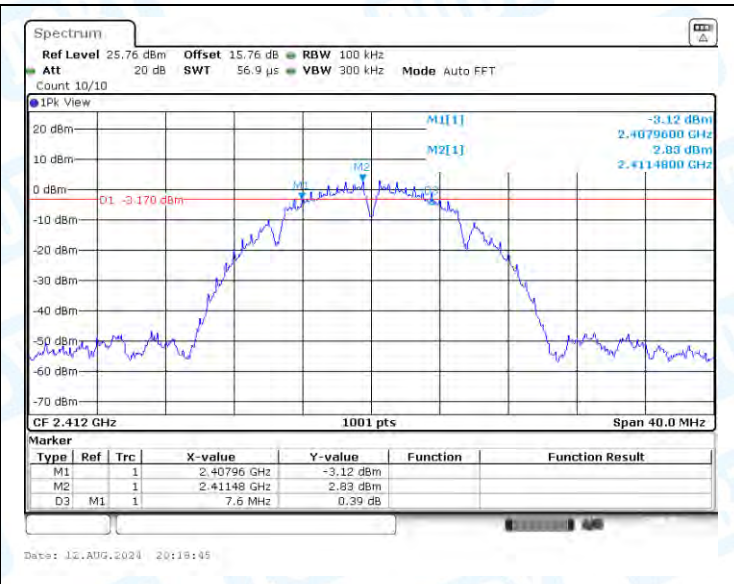
11B-Ant2-2412-PASS
