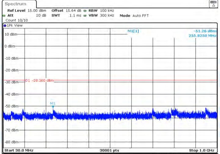
11B-Ant1-2462-30~1000-PASS
