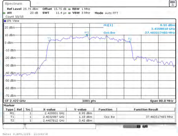
11AX40-CDD-Ant2-2422
