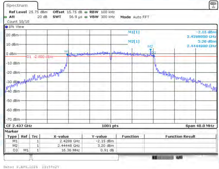
11G-CDD-Ant2-2437-PASS
