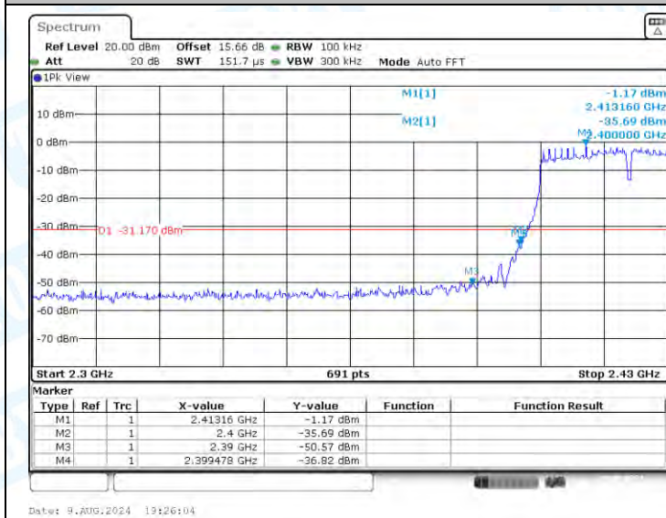
11N40-CDD-Ant1-2422-PASS
