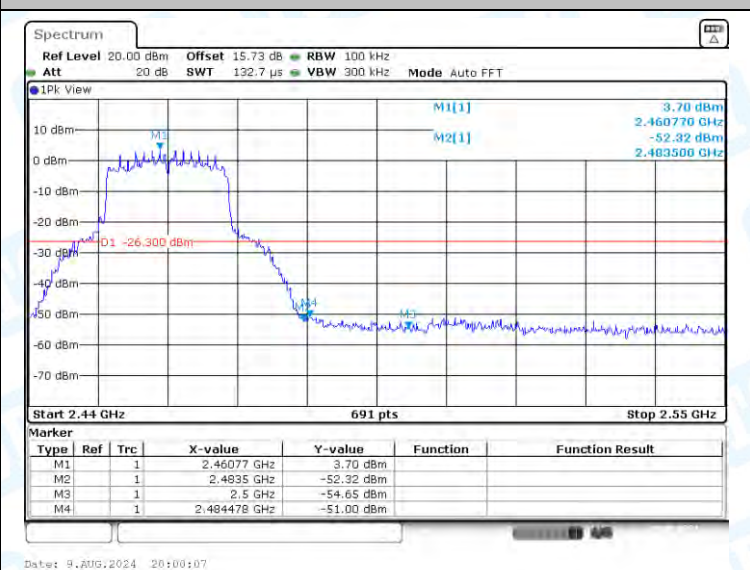
11AX20-CDD-Ant2-2462-PASS
