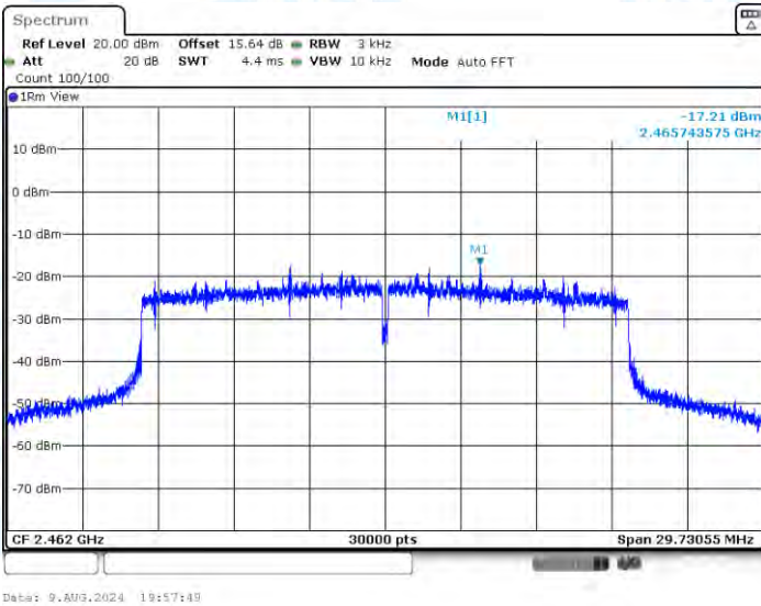
11AX20-CDD-Ant1-2462-PASS
