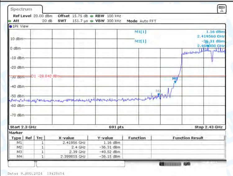
11N40-CDD-Ant2-2422-PASS
