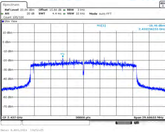
11AX20-CDD-Ant1-2437-PASS
