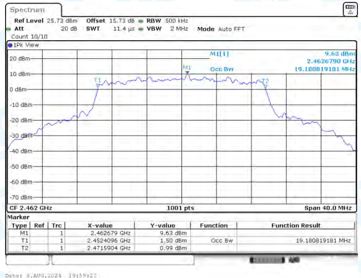
11AX20-CDD-Ant2-2462
