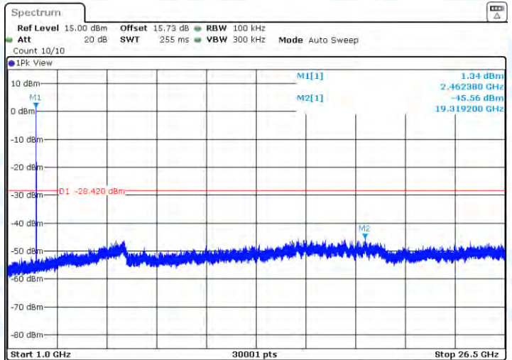
11B-Ant2-2462-0~Reference-PASS
