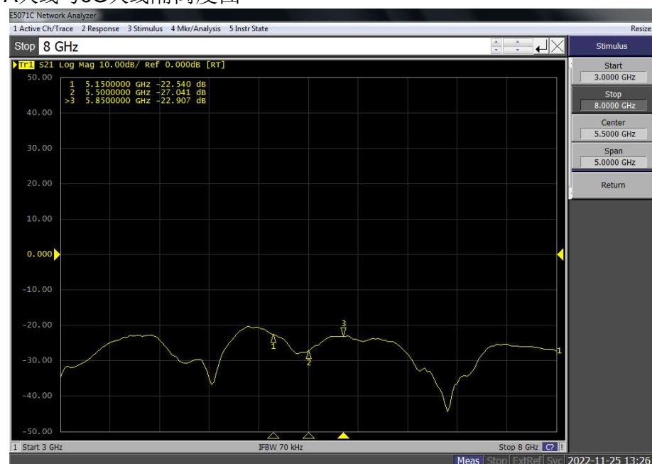
Isolation of antenna A and 5G antenna
