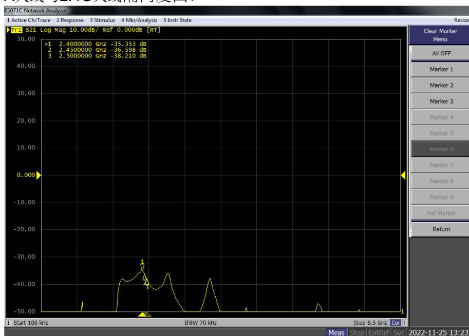
Isolation of antenna A and 2.4G antenna
