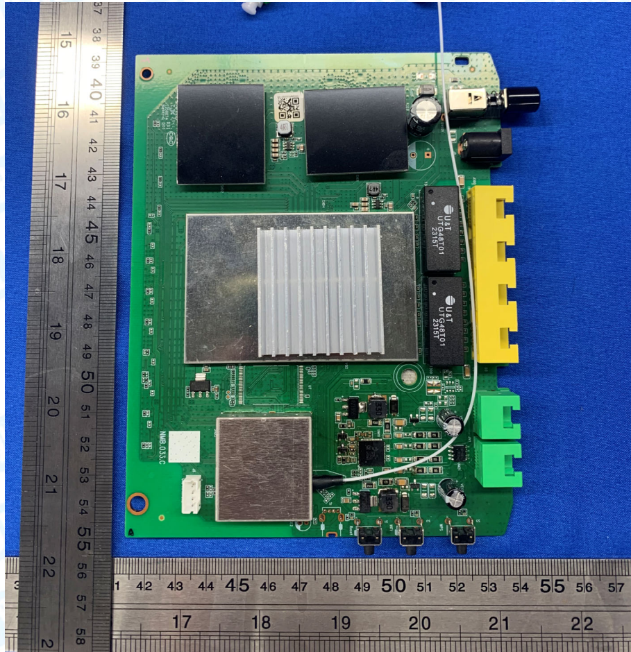
Photo 14 Appearance of PCB
