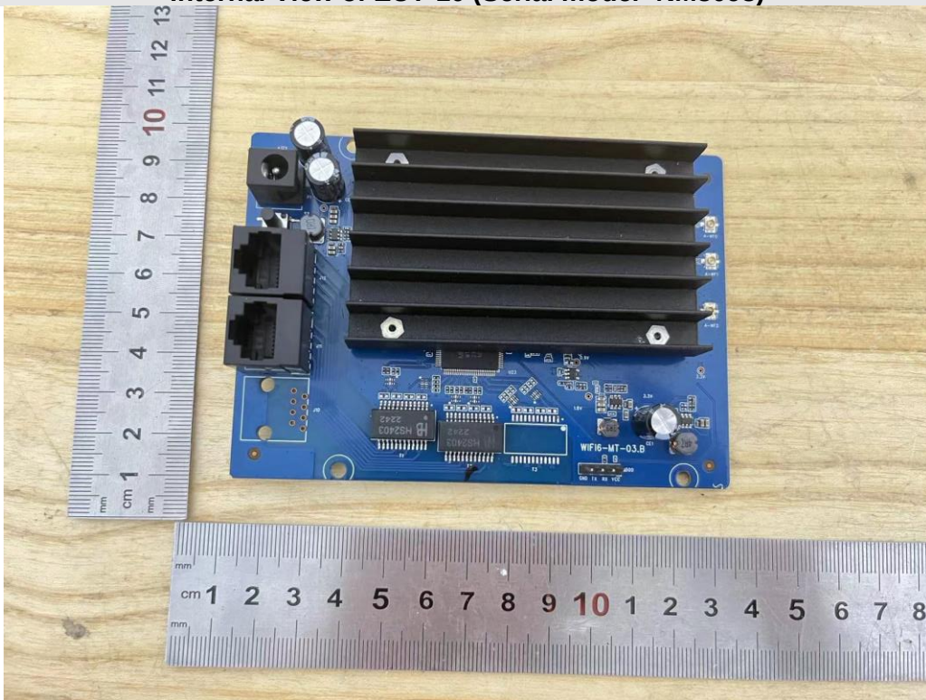
Internal View of EUT-10 (Serial model- NM3098)
