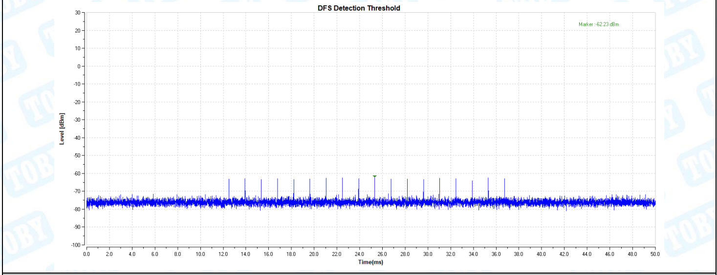
11AX80-5530-Type0-PASS
