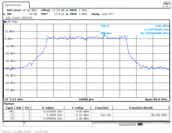
11AX40-5510-PASS
