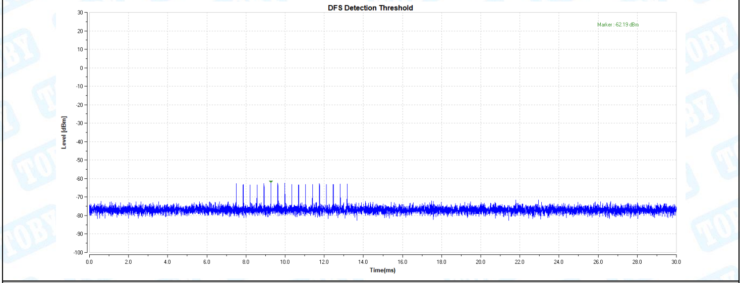
11AX20-5500-Type3-PASS
