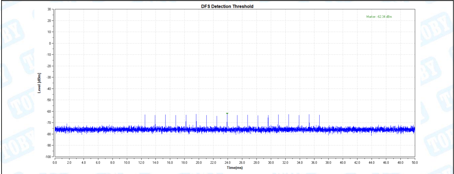
11AX160-5570-Type0-PASS
