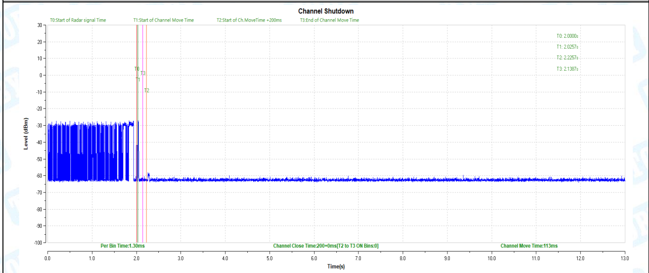
11AX160_5570
