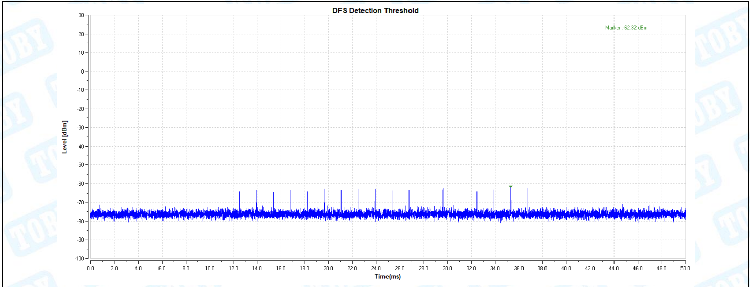
11AX40-5510-Type0-PASS
