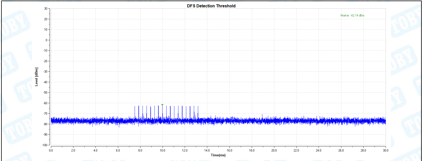
11AX160-5250-Type3-PASS
