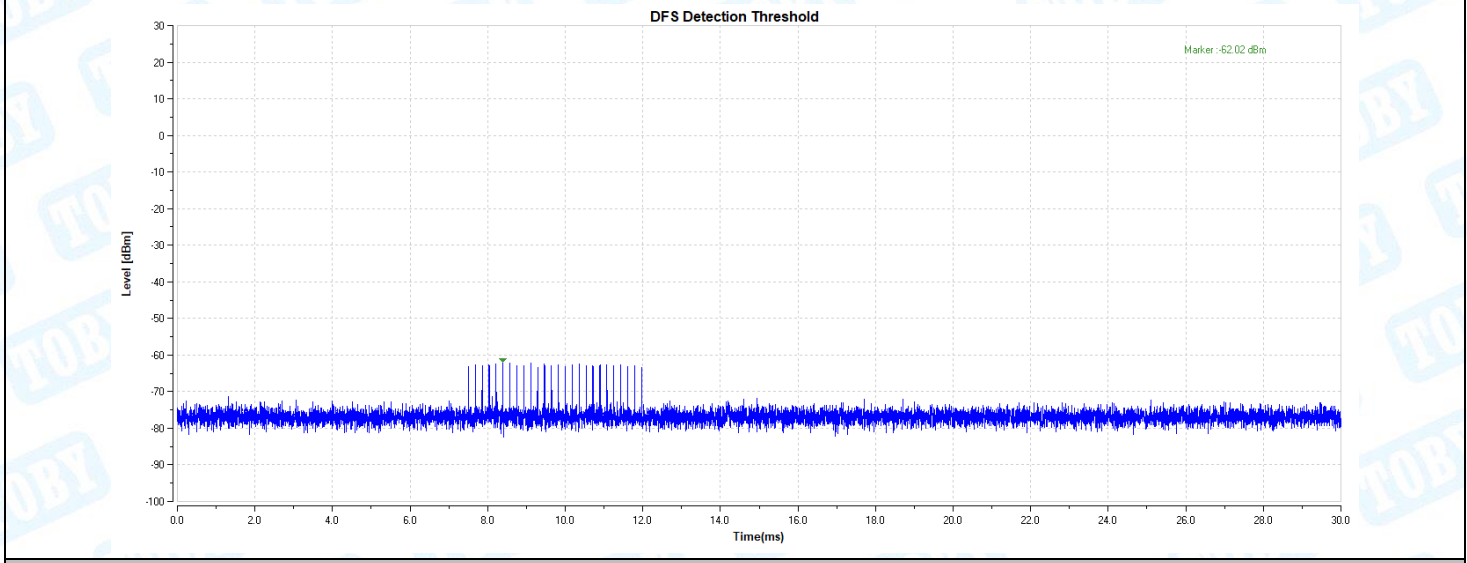
11AX40-5510-Type2-PASS
