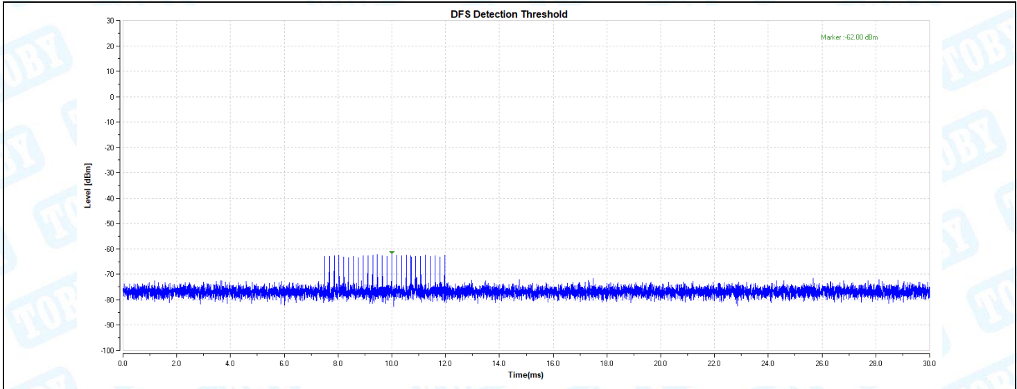
11AX80-5290-Type2-PASS
