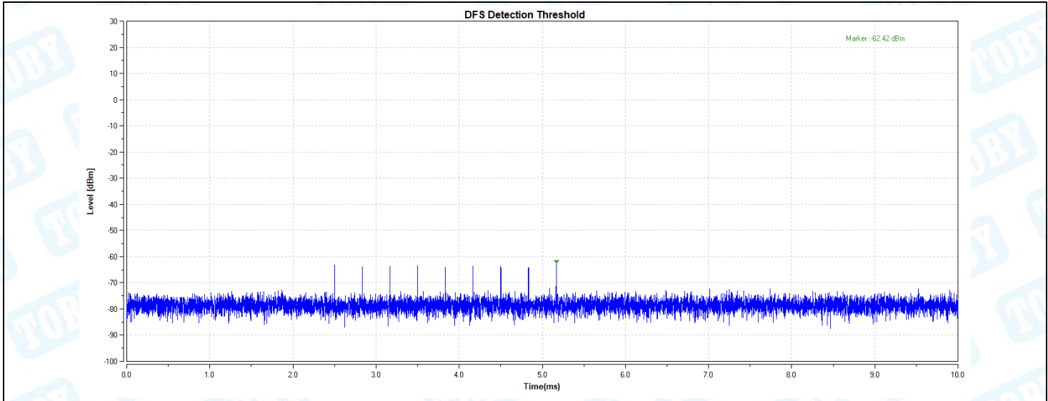
11AX160-5250-Type6-PASS
