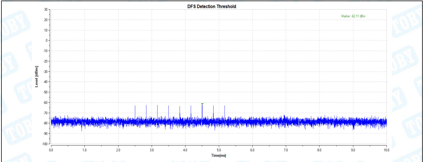
11AX20-5260-Type6-PASS
