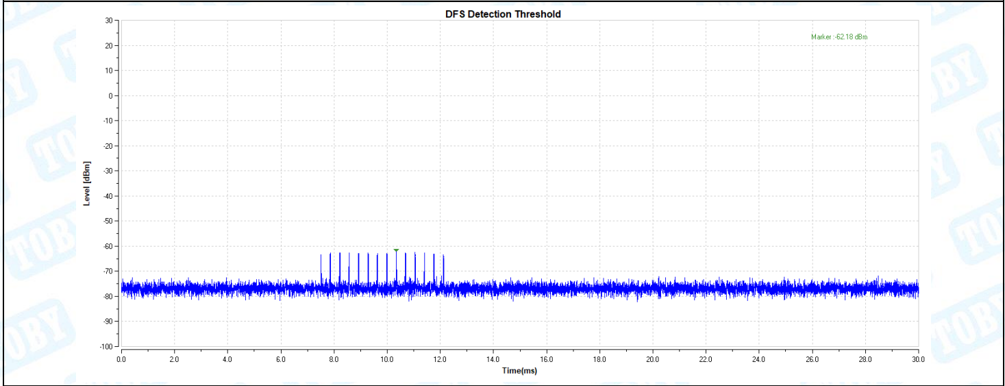
11AX80-5290-Type4-PASS
