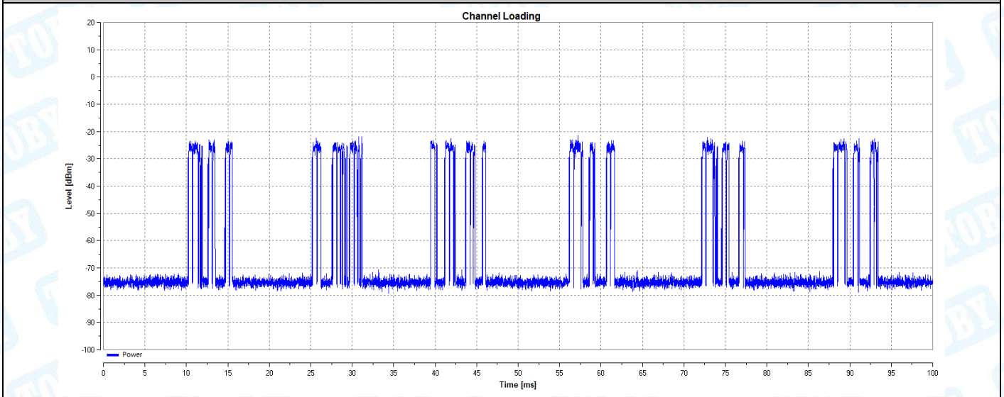
11AX160-5570-PASS
