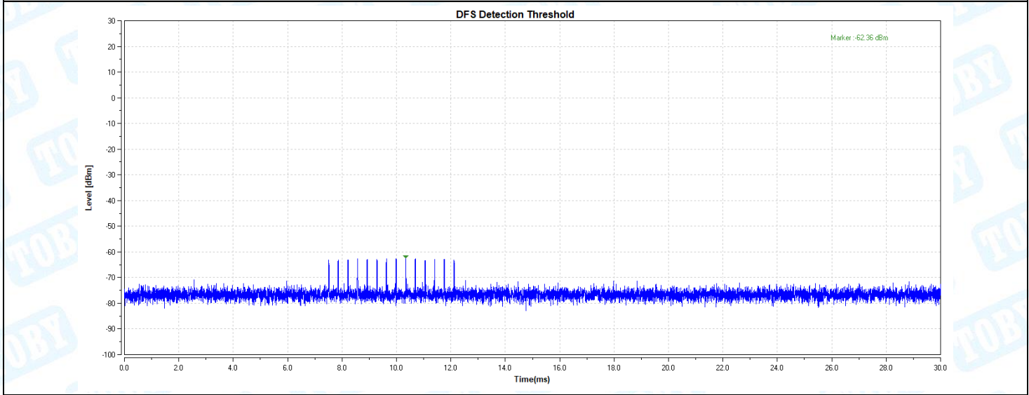
11AX160-5570-Type4-PASS
