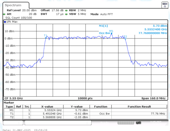
11AX80-5530-PASS
