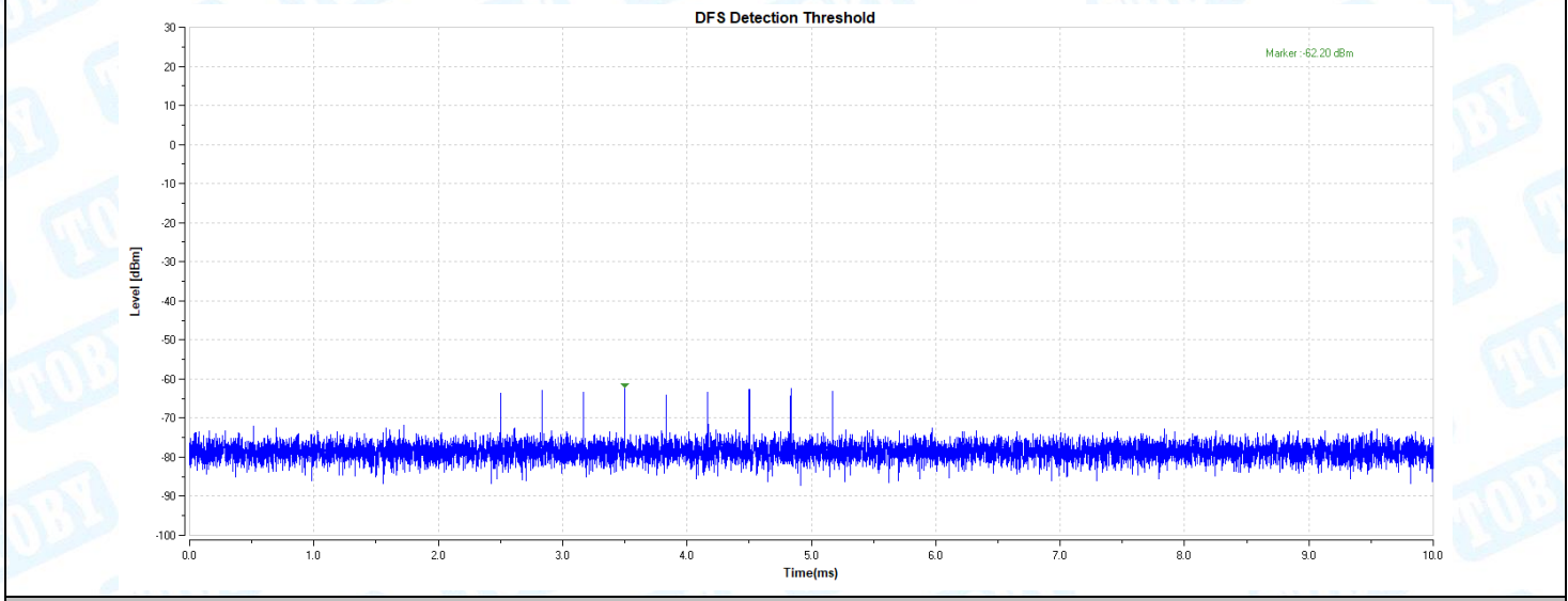
11AX80-5530-Type6-PASS
