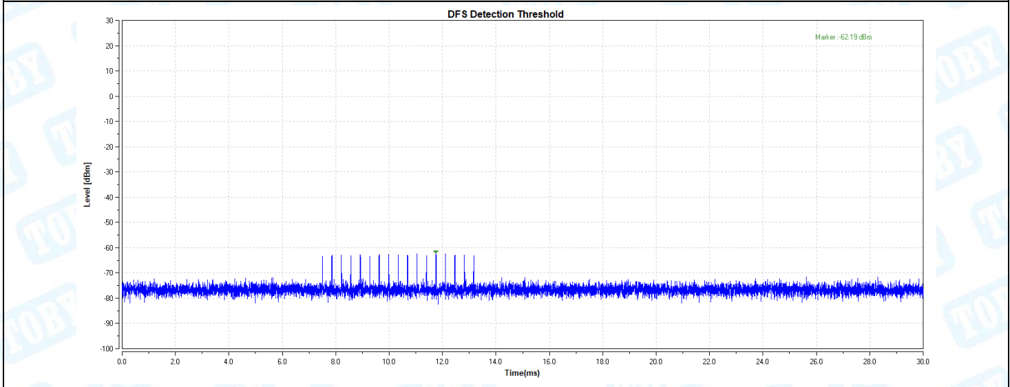
11AX160-5570-Type3-PASS
