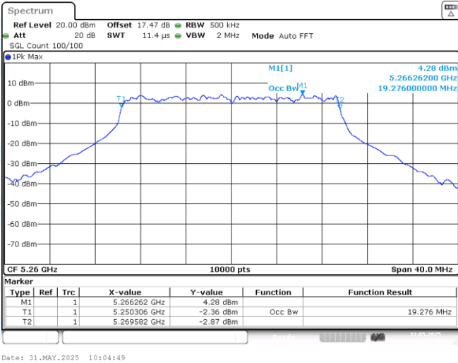
11AX20-5260-PASS
