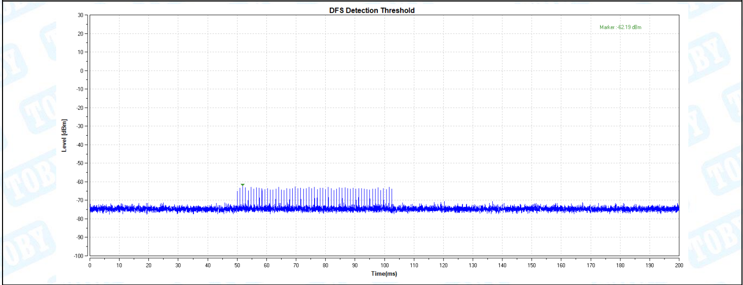
11AX160-5570-Type1-PASS
