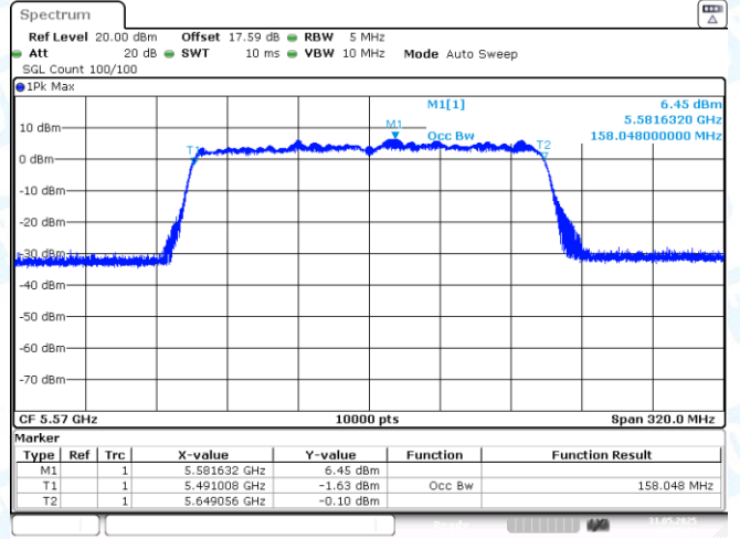
11AX160-5570-PASS
