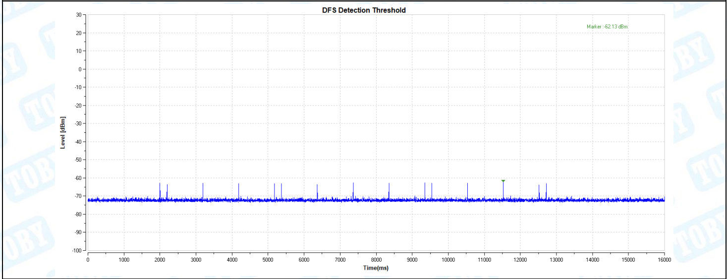
11AX160-5250-Type5-PASS
