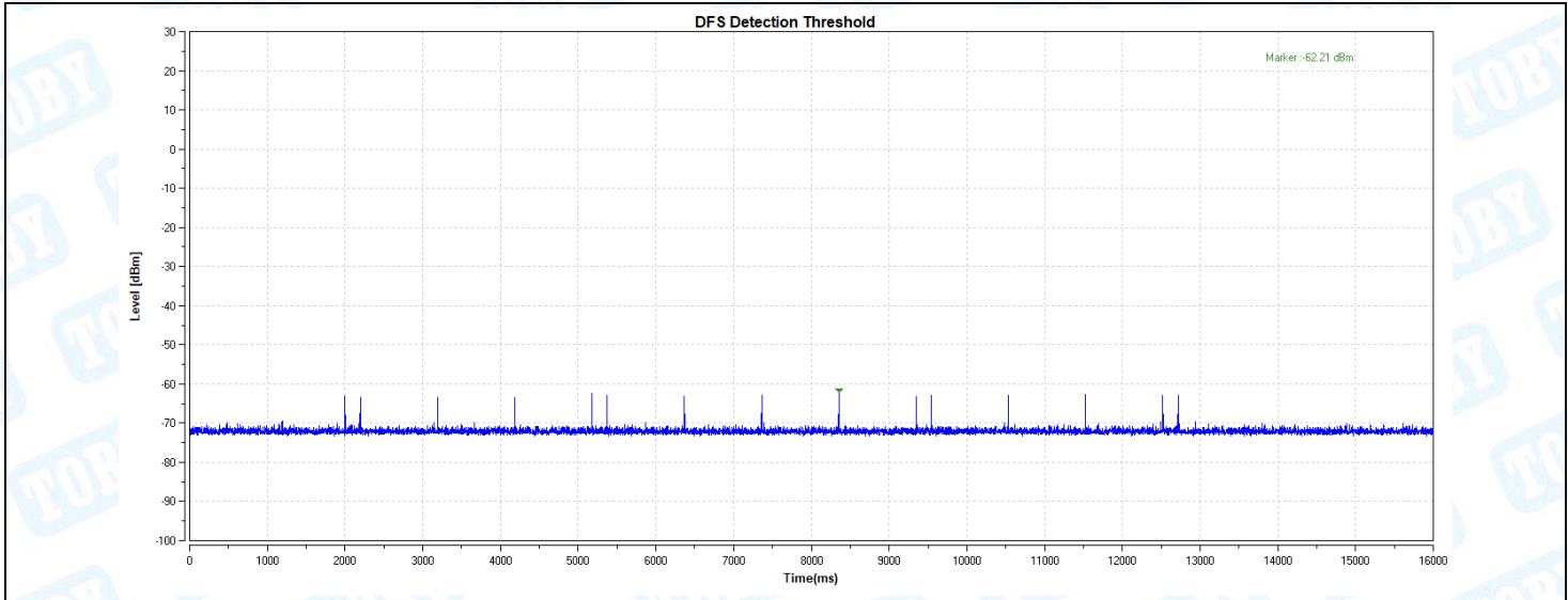
11AX160-5570-Type5-PASS
