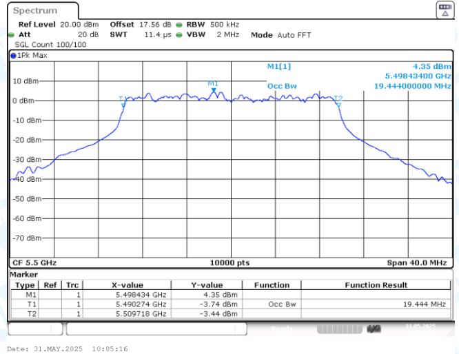
11AX20-5500-PASS
