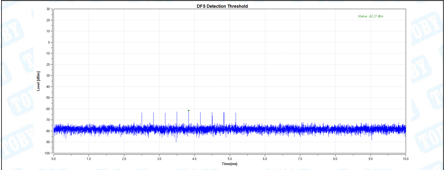
11AX160-5570-Type6-PASS
