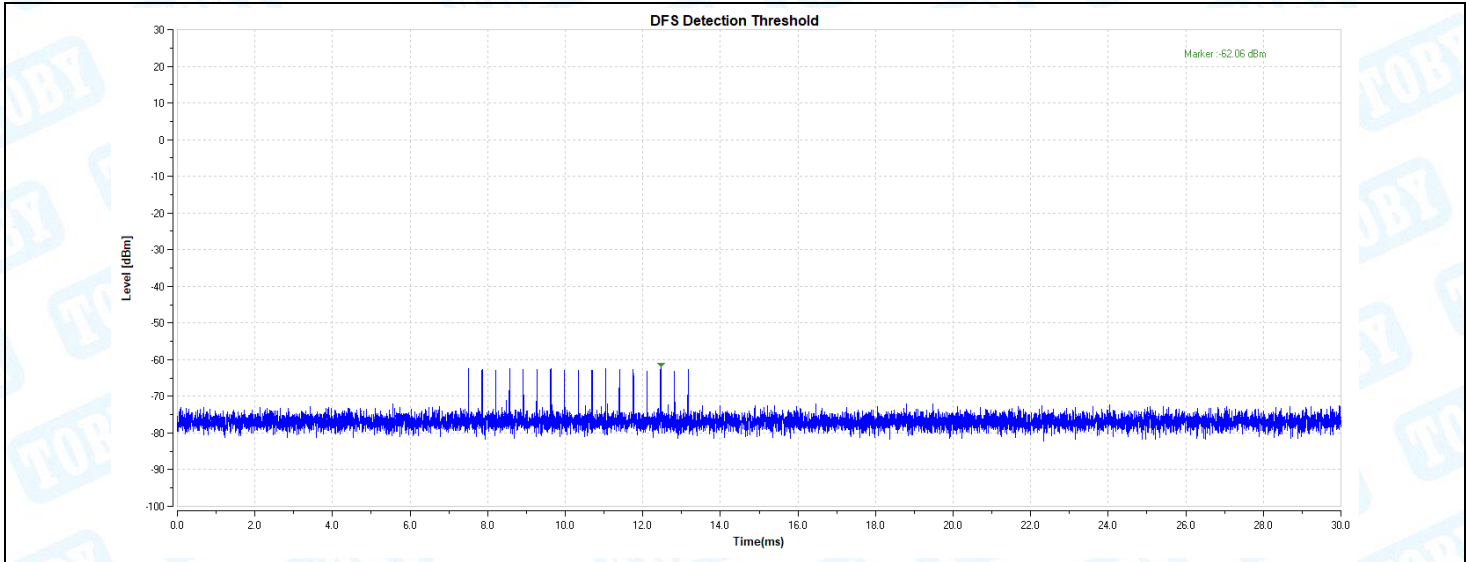
11AX20-5260-Type3-PASS
