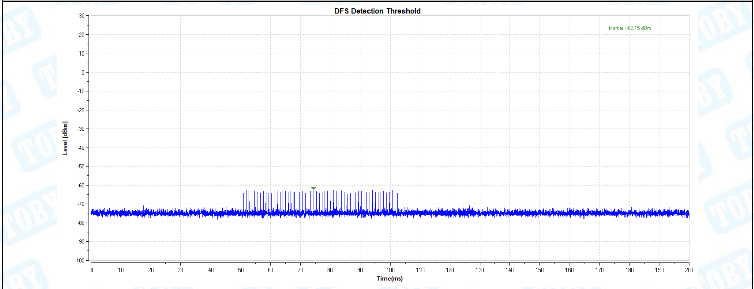
11AX20-5260-Type1-PASS
