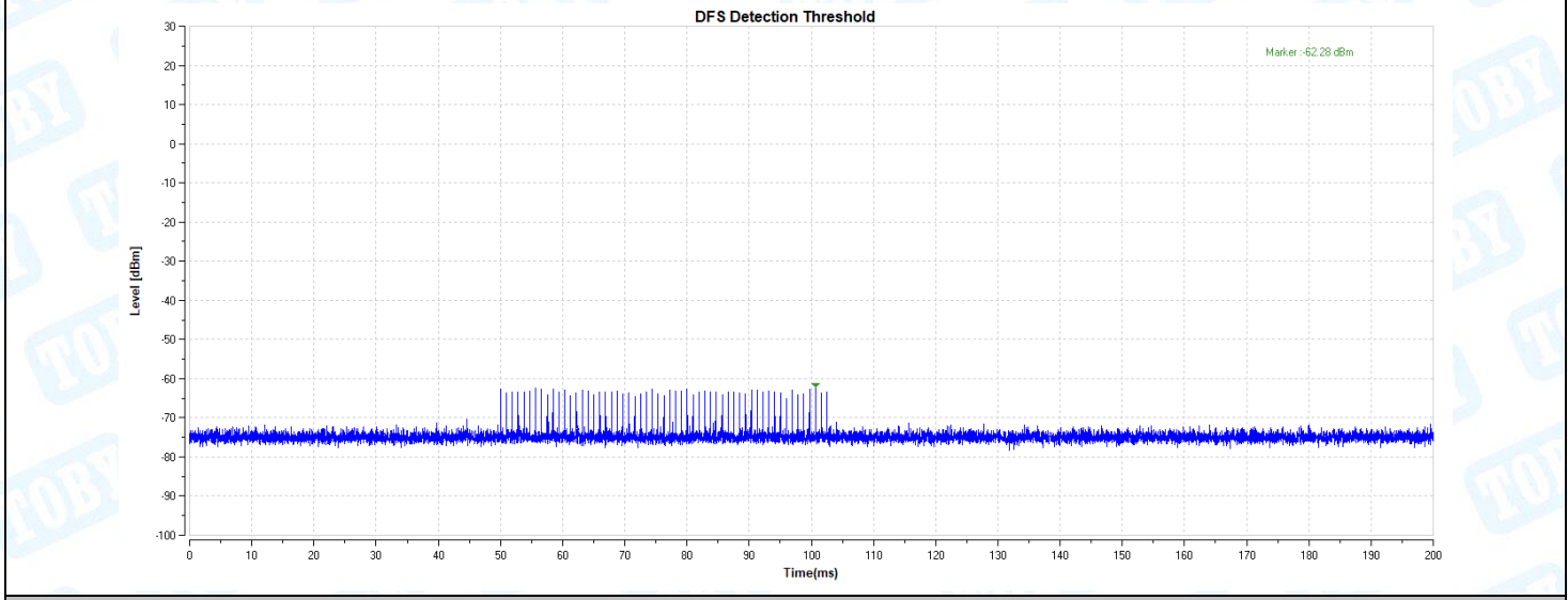
11AX40-5510-Type1-PASS
