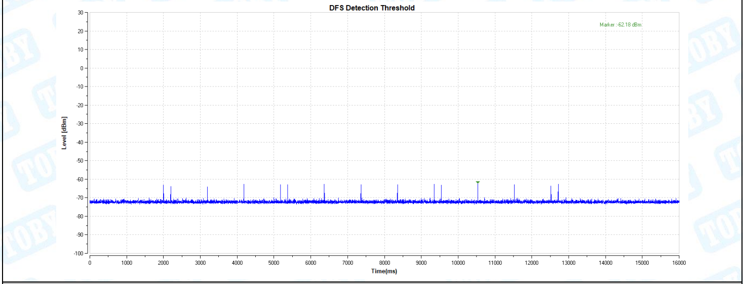
11AX80-5530-Type5-PASS
