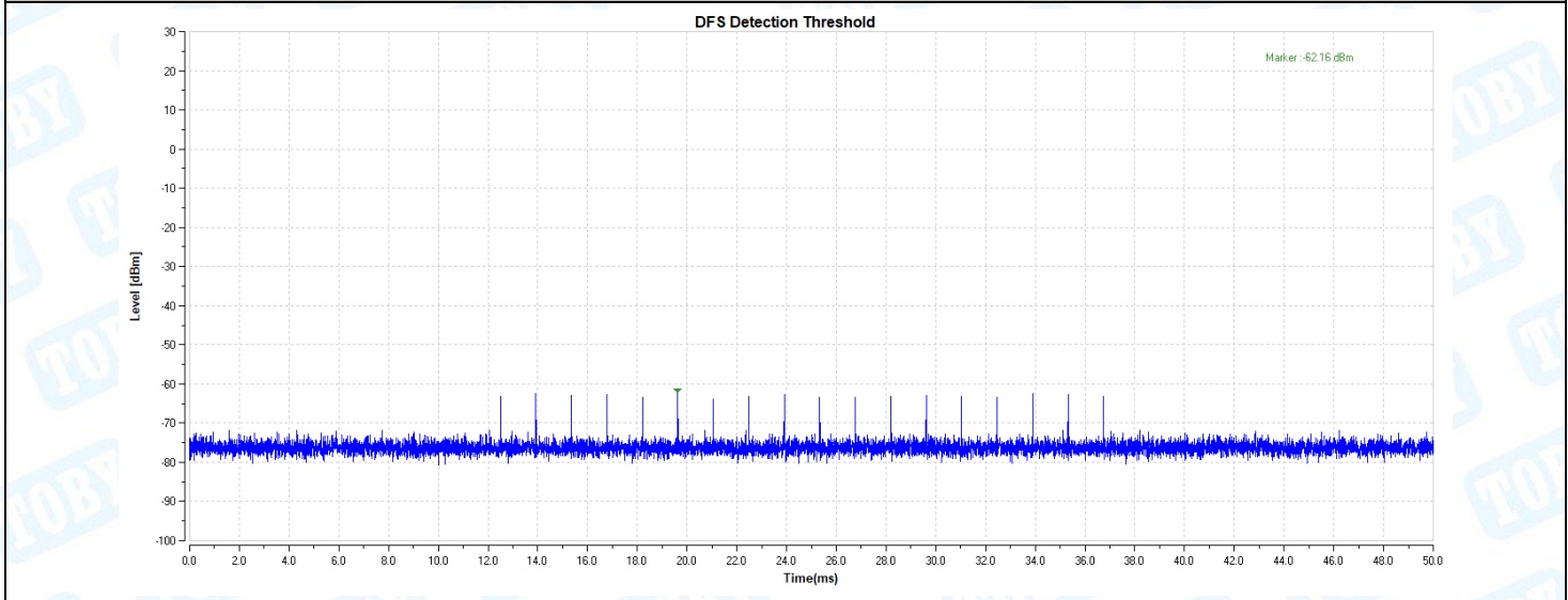
11AX80-5290-Type0-PASS
