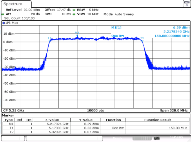
11AX160-5250-PASS
