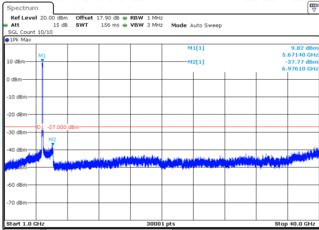
11AC80-CDD-Ant1-5690-1000~40000-PASS
