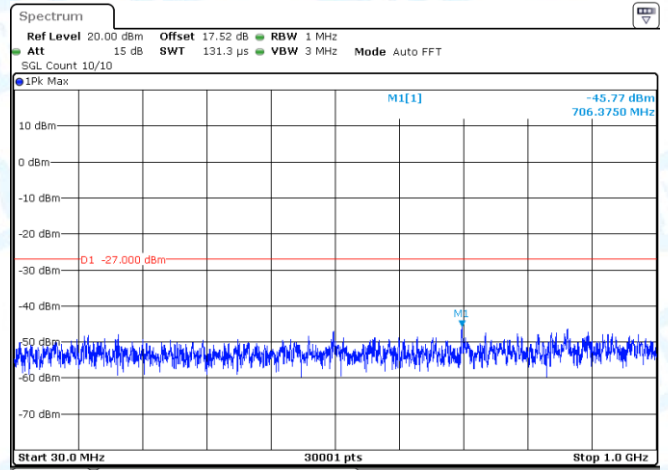
11AC40-CDD-Ant2-5310-30~1000-PASS
