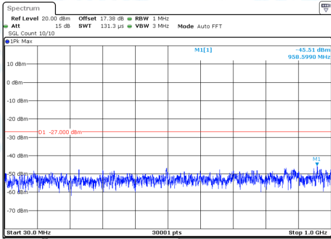
11AC40-CDD-Ant1-5190-30~1000-PASS
