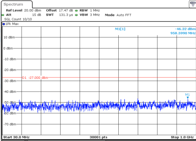
11AC160-CDD-Ant1-5250-30~1000-PASS
