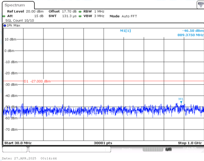
11AC80-CDD-Ant1-5610-30~1000-PASS
