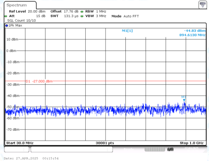
11AC80-CDD-Ant2-5610-30~1000-PASS
