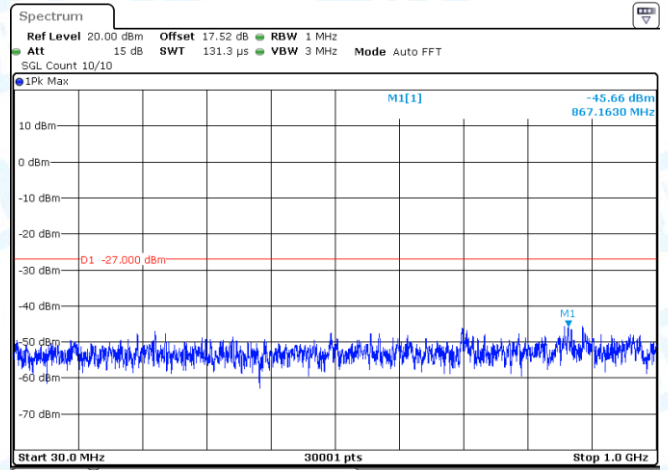
11AX20-CDD-Ant2-5280-30~1000-PASS
