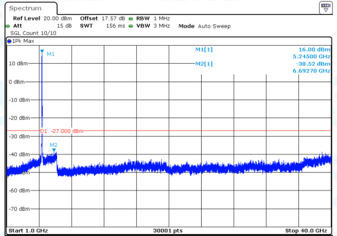
11AC40-CDD-Ant2-5230-1000~40000-PASS
