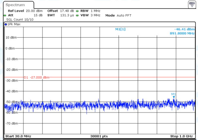
11AC40-CDD-Ant2-5190-30~1000-PASS
