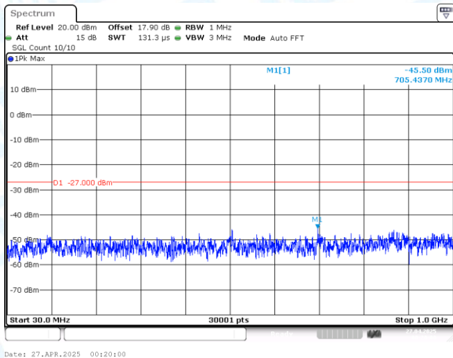
11AC80-CDD-Ant1-5690-30~1000-PASS
