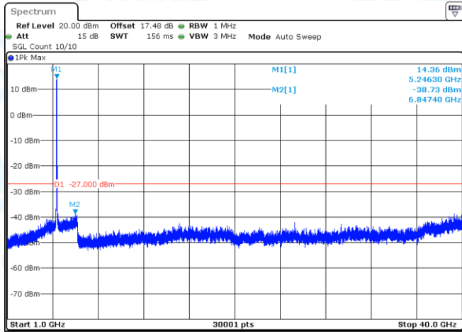
11AC40-CDD-Ant1-5230-1000~40000-PASS
