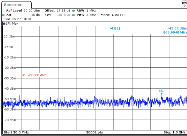
11AX20-CDD-Ant1-5200-30~1000-PASS
