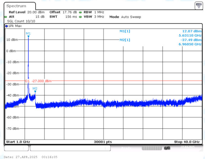
11AC80-CDD-Ant2-5610-1000~40000-PASS
