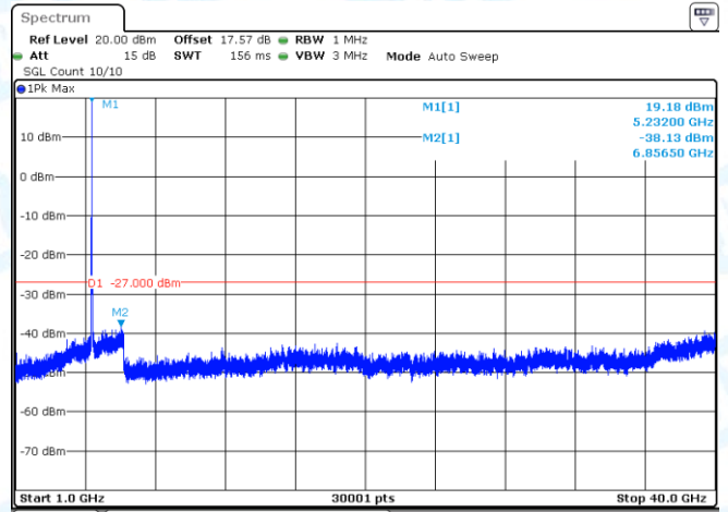
11AX20-CDD-Ant2-5240-1000~40000-PASS
