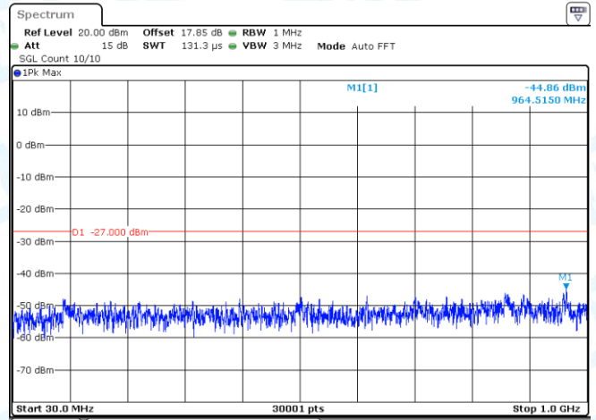
11AC40-CDD-Ant2-5710-30~1000-PASS
