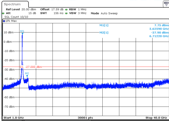
11AC160-CDD-Ant1-5570-1000~40000-PASS
