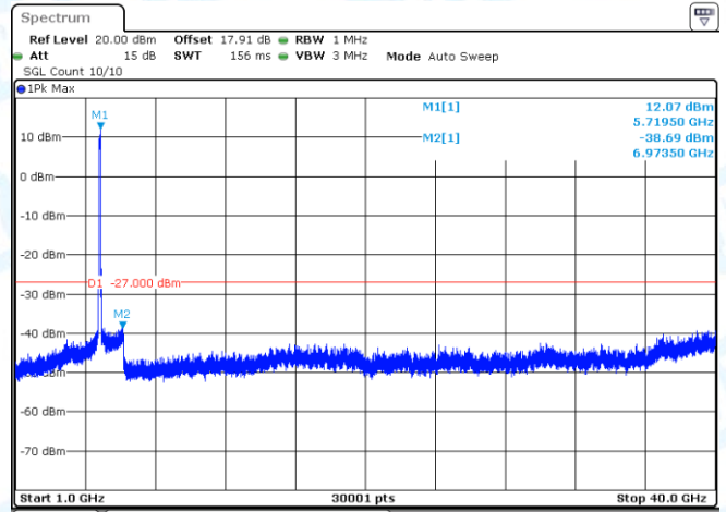
11AC80-CDD-Ant2-5690-1000~40000-PASS
